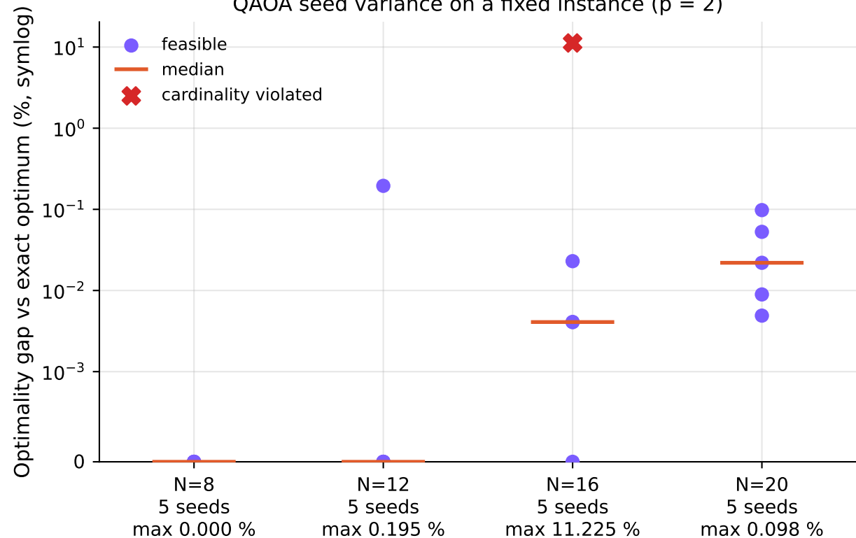
QAOA seed variance on a fixed instance ( p = 2 )
