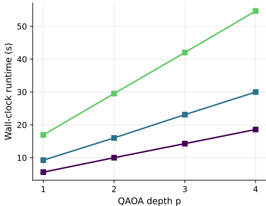
Cost of depth (lightning.gpu)
