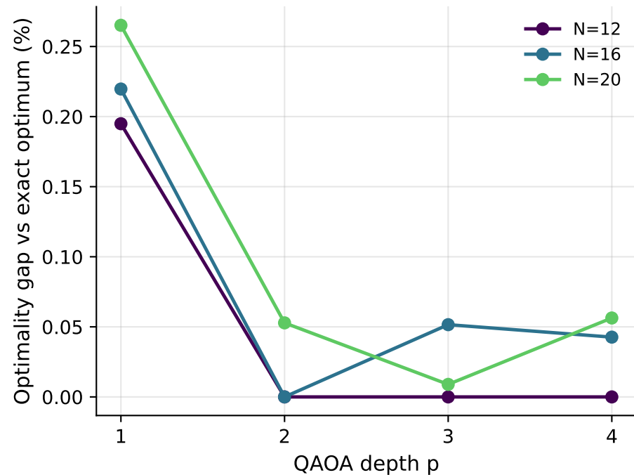
Solution quality vs depth
