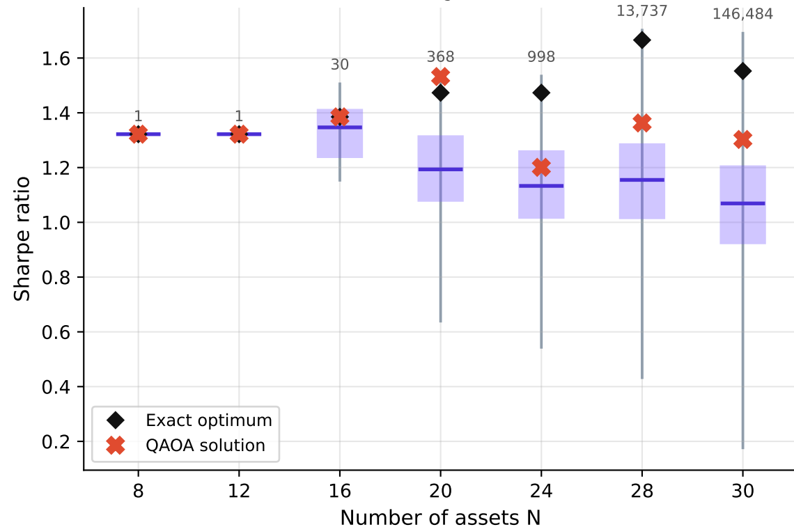
Sharpe ratios within a 0.1% optimality gap (box = IQR, whisker = full range, label = solutions in band)
