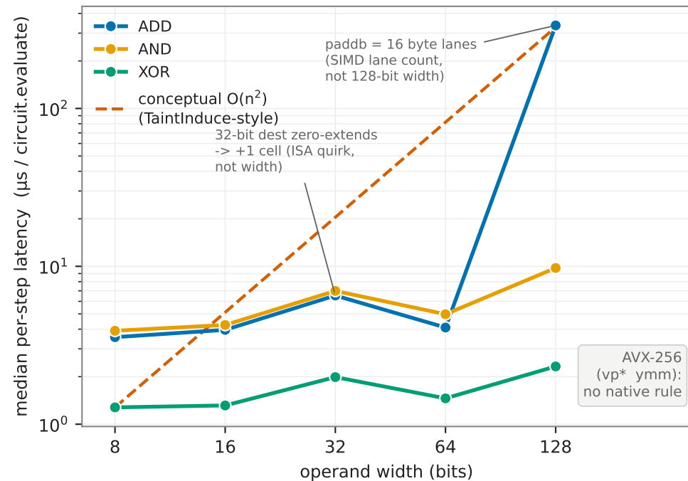
(a) Per-step cost vs operand width
