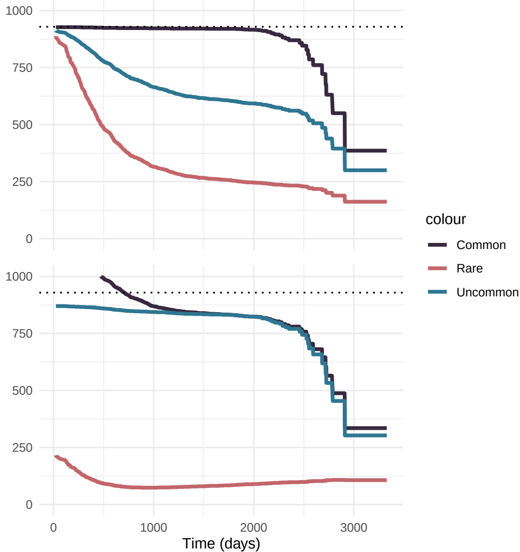
Effective Sample Size of Predictions
