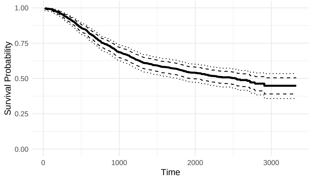
Cox model prediction with pointwise confidence interval
