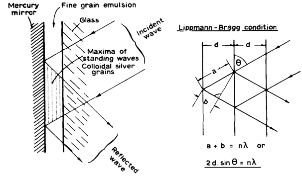
FIG. 5: Gabriel Lippmann's method of photography
