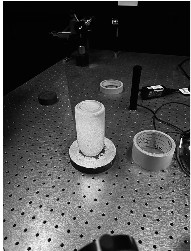
FIG. 19: Photo of the spotted pattern from the dusty aspheric lens. The rounded features on the interference pattern is as a result of diffraction of smaller particles on lens, not a feature of the desired interference.
