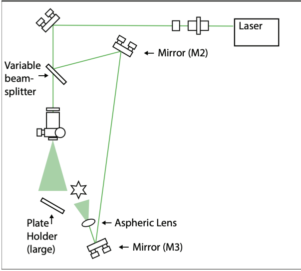
FIG. 8: Similar set up to the reflection hologram except the object is now moved in front of the plate. Again blockers were used to ensure the paths do not cross paths, even after spread out before they hit the plate.
