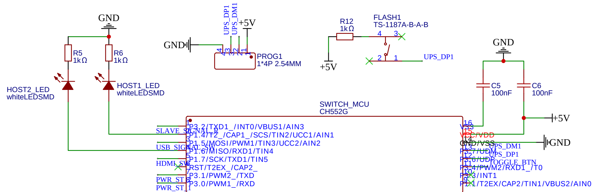
Switch Control MCU
