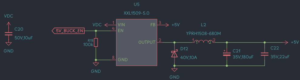
5V converter
