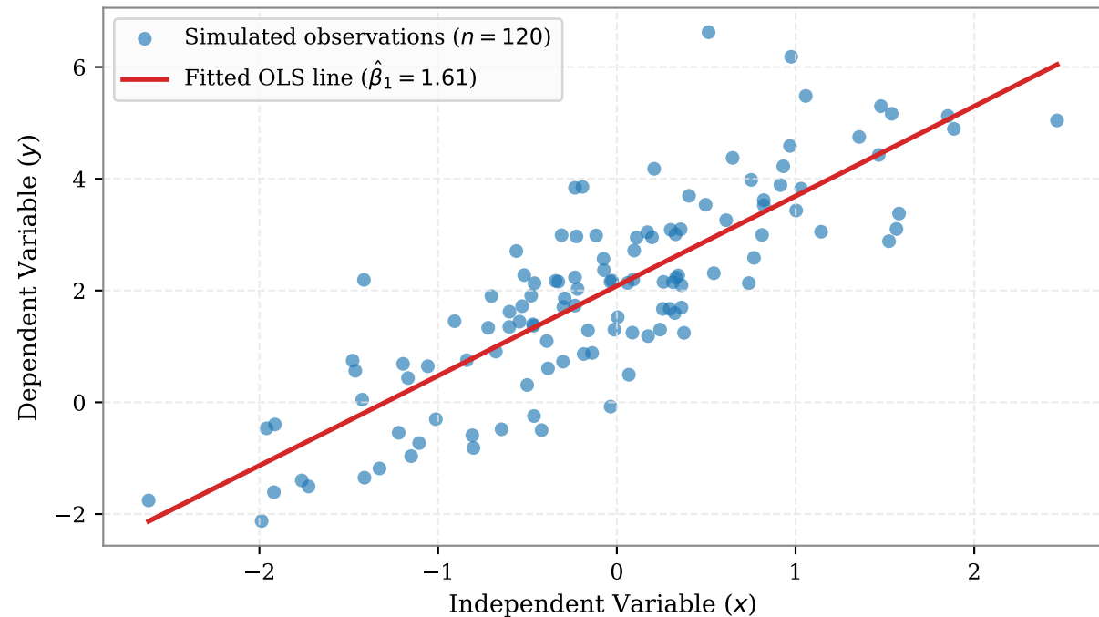
Linear Regression Fit on Simulated DGP Data
