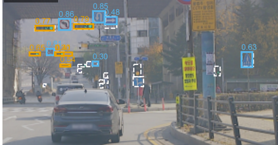
12 detections
