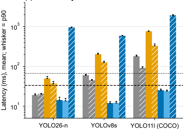
(a) Windows: Ryzen 5 9600X + RTX 5070
