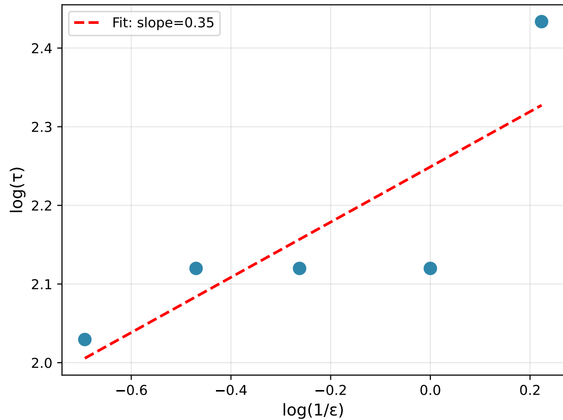
\varepsilon -Scaling Test (M=4) Slope=0.35, R^2=0.677
