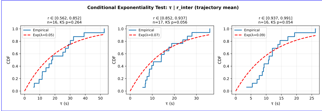
Figure 2: Conditional exponentiality diagnostic. Unconditional inter-commit interval distributions can appear heavy-tailed. Conditioning on narrow bins of inter-module coherence r_{\text{inter}} among observed commits yields approximately exponential waiting times within each bin (Kolmogorov-Smirnov test), consistent with a mixture-of-exponentials interpretation in which slow drift of r(t) broadens the marginal waiting-time distribution. Because this analysis conditions on observed hits, it should be read as a diagnostic rather than a full survival-model validation.
