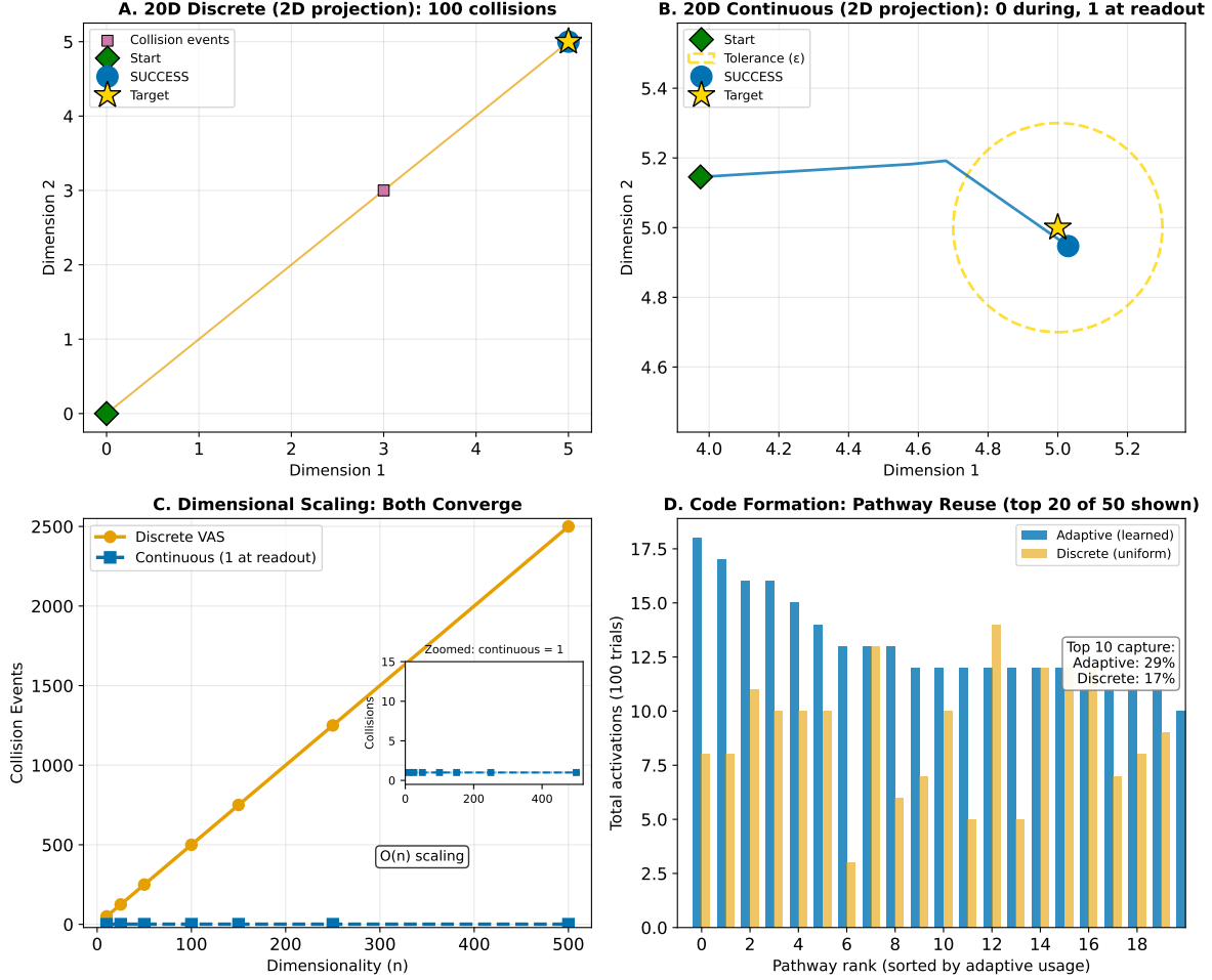
Figure 1: Collision-Free Computation Through High-Dimensional Dynamics. (A) 20D discrete VAS with independent transitions (2D projection; best case for discrete): greedy search converges in 100 collision events. Each collision pays Landauer cost k_B T \ln 2 . Pink squares show state snapshots (collisions counted per-dimension, not per-snapshot). Note: this quantifies collision cost only; both substrates pay maintenance costs (clock power, ion pumps, synaptic homeostasis). (B) 20D continuous gradient descent (2D projection): converges with zero collision events during evolution (cost paid only at final measurement = 1 k_B T \ln 2 ). The key distinction is collision count , not solvability—discrete accumulates O(n) irreversible transitions; continuous pays only once. (C) Dimensional scaling with independent transitions (best case for discrete): collision count scales as O(n) . Panel shows fixed target displacement of 5 units/dimension, giving slope \approx 5 (at n = 10 : 50 collisions; at n = 500 : 2500 collisions). Table 2 uses randomized start/target ranges with expected displacement \approx 4 , giving slope \approx 3.95 . The key result—linear scaling with dimension—is robust to parameter choice. Continuous requires only the single final readout ( \equiv 1 ) at all dimensions including biologically realistic scales ( n = 30 – 100 ). Both approaches always converge. (D) Code formation via pathway reuse: adaptive system (blue) concentrates usage on fewer pathways through Hebbian strengthening, while discrete enumeration (orange) distributes usage uniformly across all pathways. Top 10 pathways capture \sim 29\% of adaptive uses versus \sim 17\% for discrete (uniform would give 20\% ). This concentration enables efficient code formation—frequently-used pathways become reliable “symbols” for recurring task patterns.
