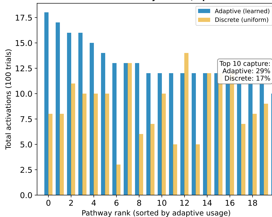
D. Code Formation: Pathway Reuse (top 20 of 50 shown)
