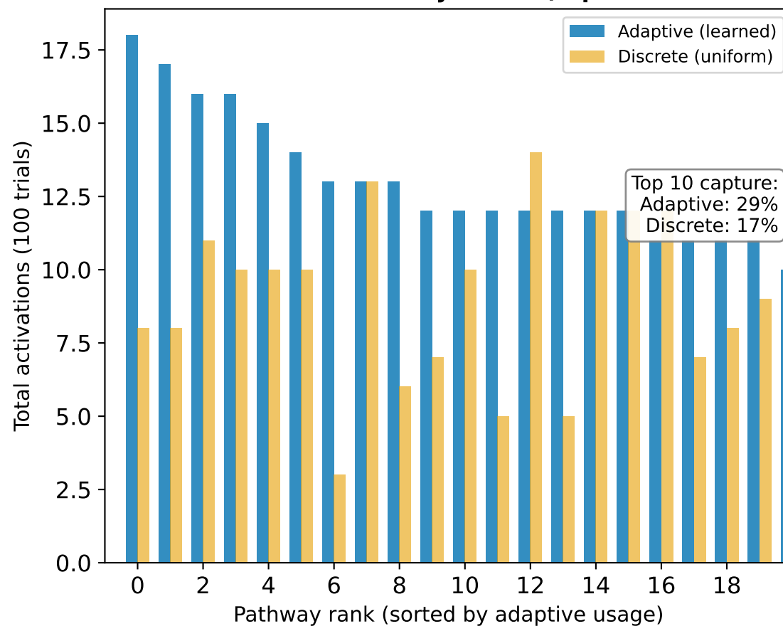
D. Code Formation: Pathway Reuse (top 20 of 50 shown)
