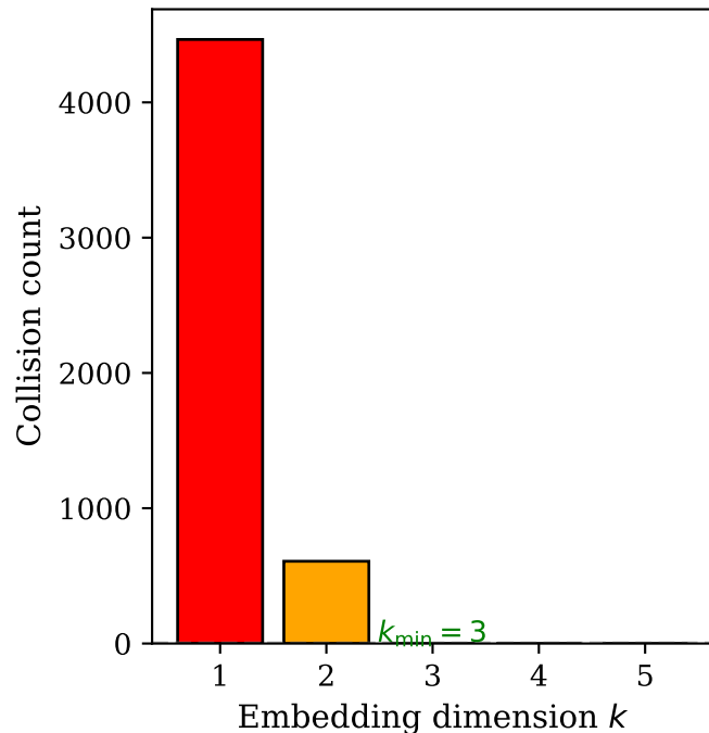
(C) Collisions vs. dimension
