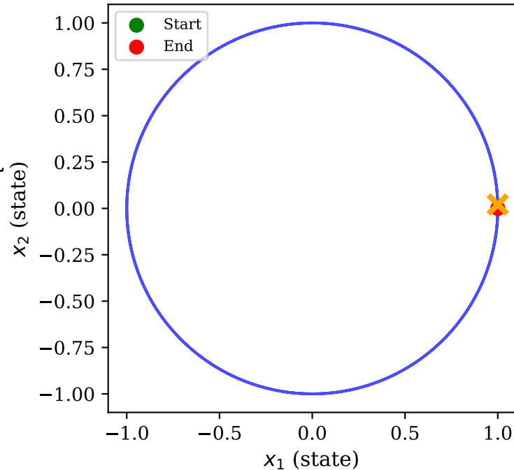
(B) k = 2 : Collisions (orange X)
