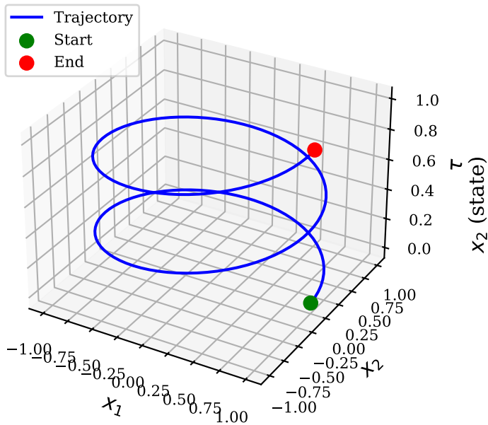
(A) k = 3 : Collision-free
