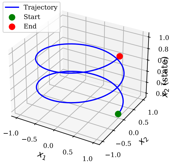
(A) k = 3 : Collision-free
