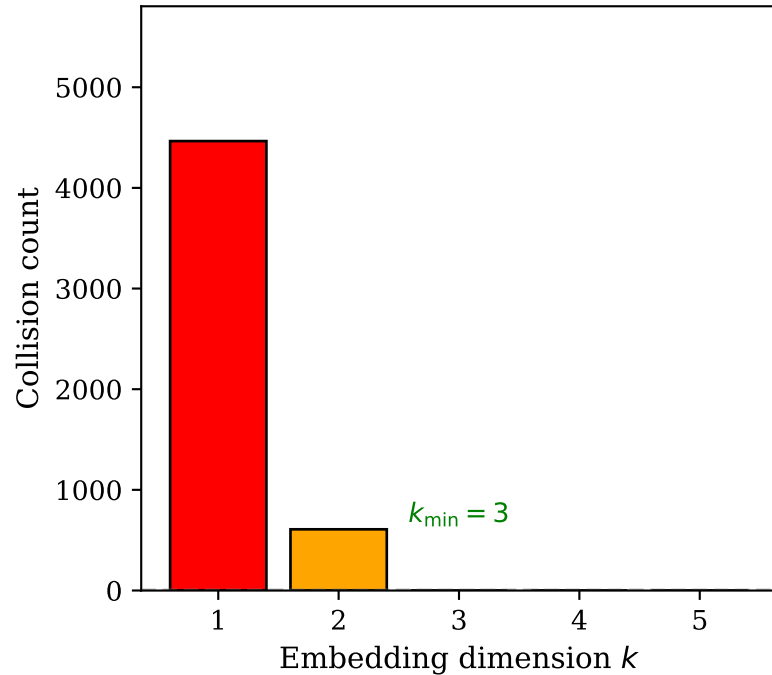
(C) Collisions vs. dimension
