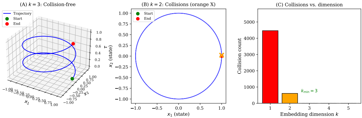
Figure 1: The self-intersection problem in dimensional collapse. (A) A helix in \mathbb{R}^3 representing a cyclic process with monotone meta-time—no self-intersections. (B) The same process projected to \mathbb{R}^2 —self-intersections occur where the trajectory crosses itself (orange X marks). (C) Self-intersection count as a function of embedding dimension k : self-intersections persist for k \leq 2 but vanish for k \geq 3 . Collision counts depend on the proximity threshold \varepsilon ; in the phase-preserving case shown here, collisions persist for all sufficiently small \varepsilon once the cycle repeats.
