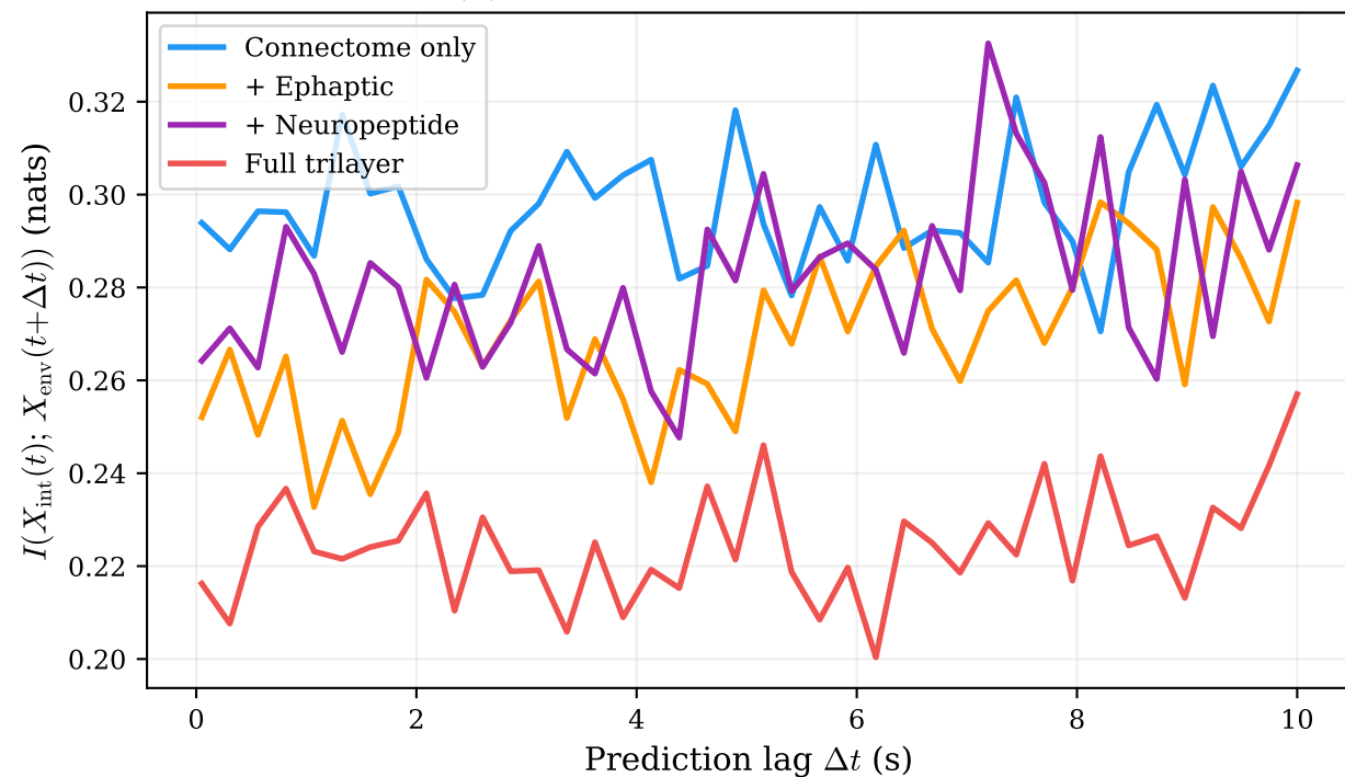
(a) Future mutual information
