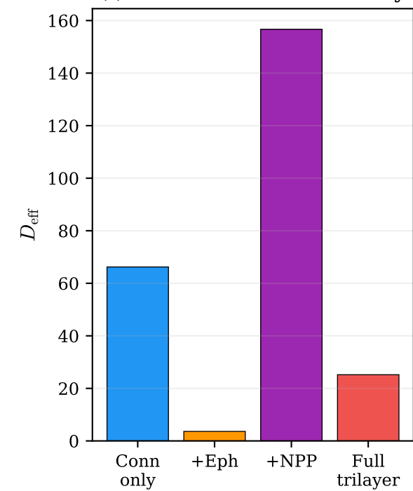
(f) Effective dimensionality
