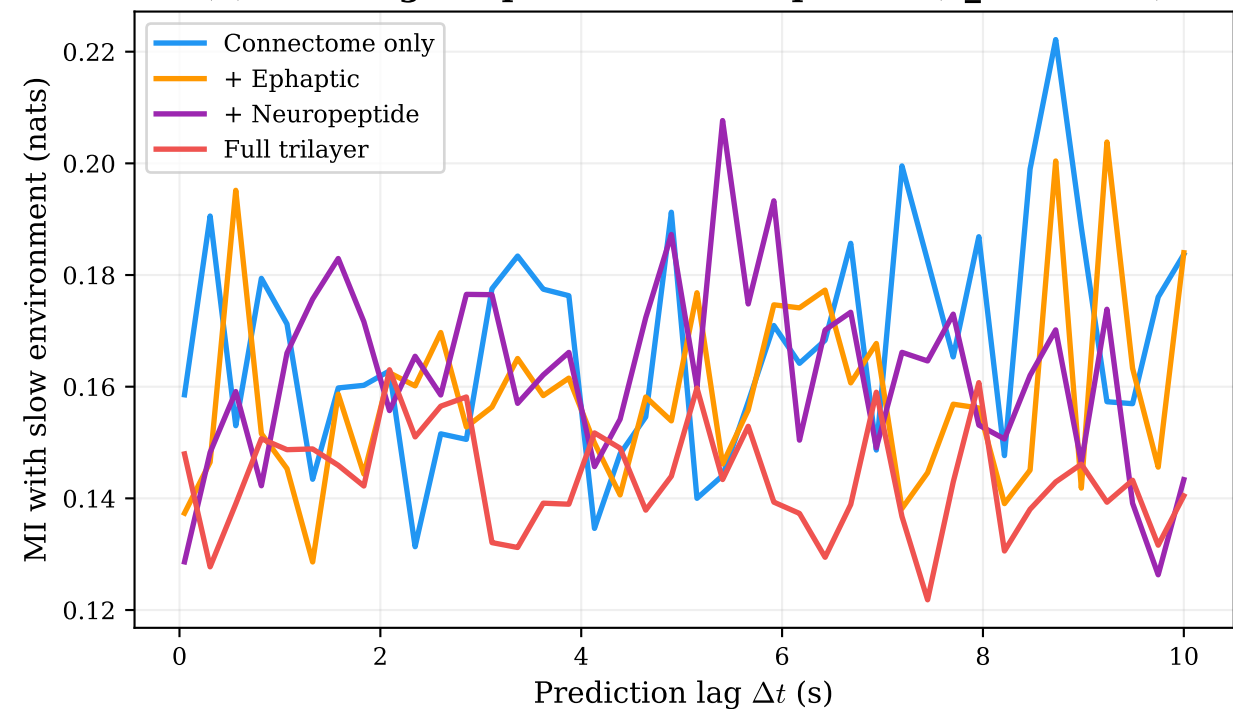
(b) Tracking the predictable component ( \tau_{\text{env}} = 10\text{s} )
