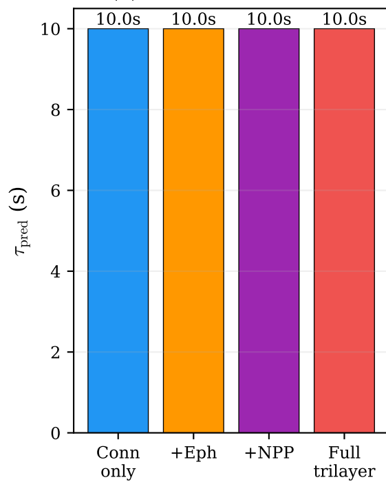
(c) Prediction horizon
