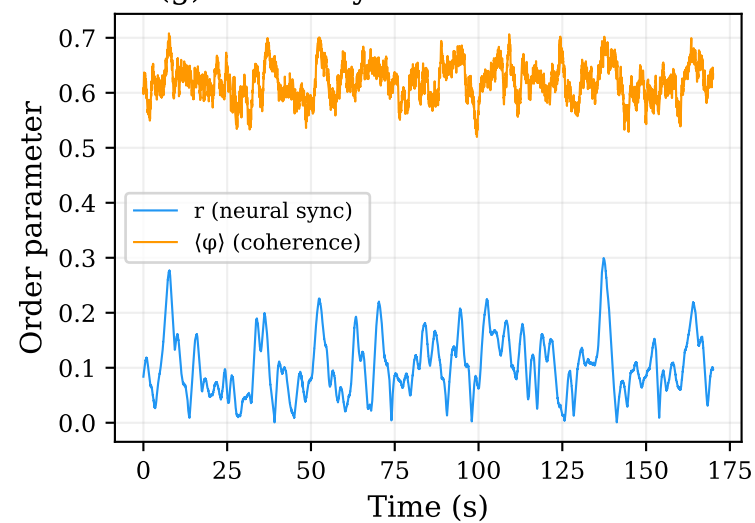
(g) Neural sync tracks coherence
