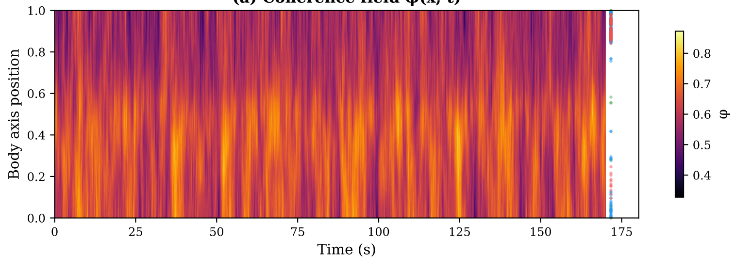
(a) Coherence field \varphi(x, t)
