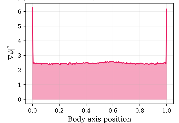
(e) Surface tension (coherence boundaries)
