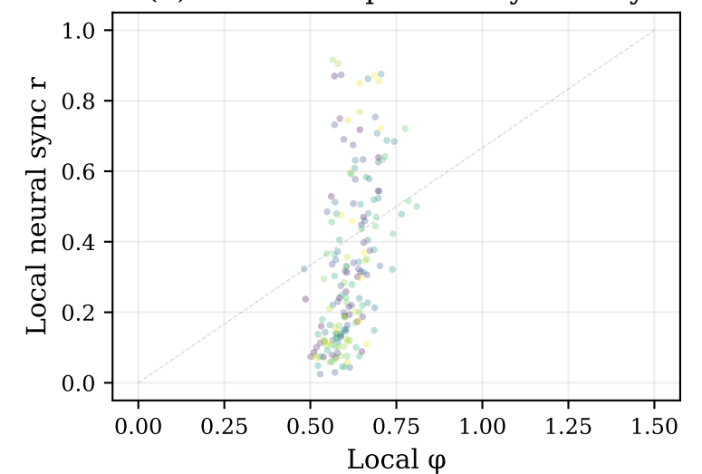
(h) Coherence predicts synchrony
