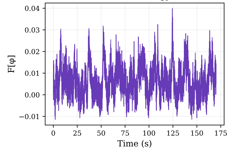
(b) Free energy
