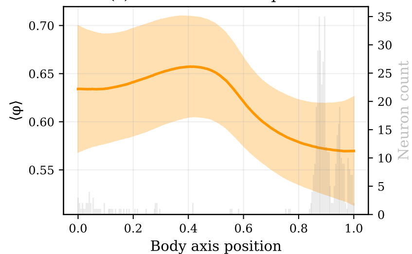
(c) Mean coherence profile
