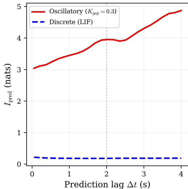
(a) Future mutual information
