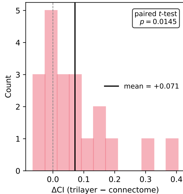
b) Paired difference
