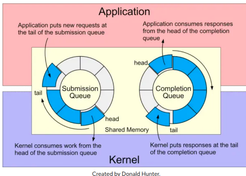
Figure 4.2: io_uring 's submission and completion queues, shared between the application and the kernel. Diagram by Donald Hunter [15].
