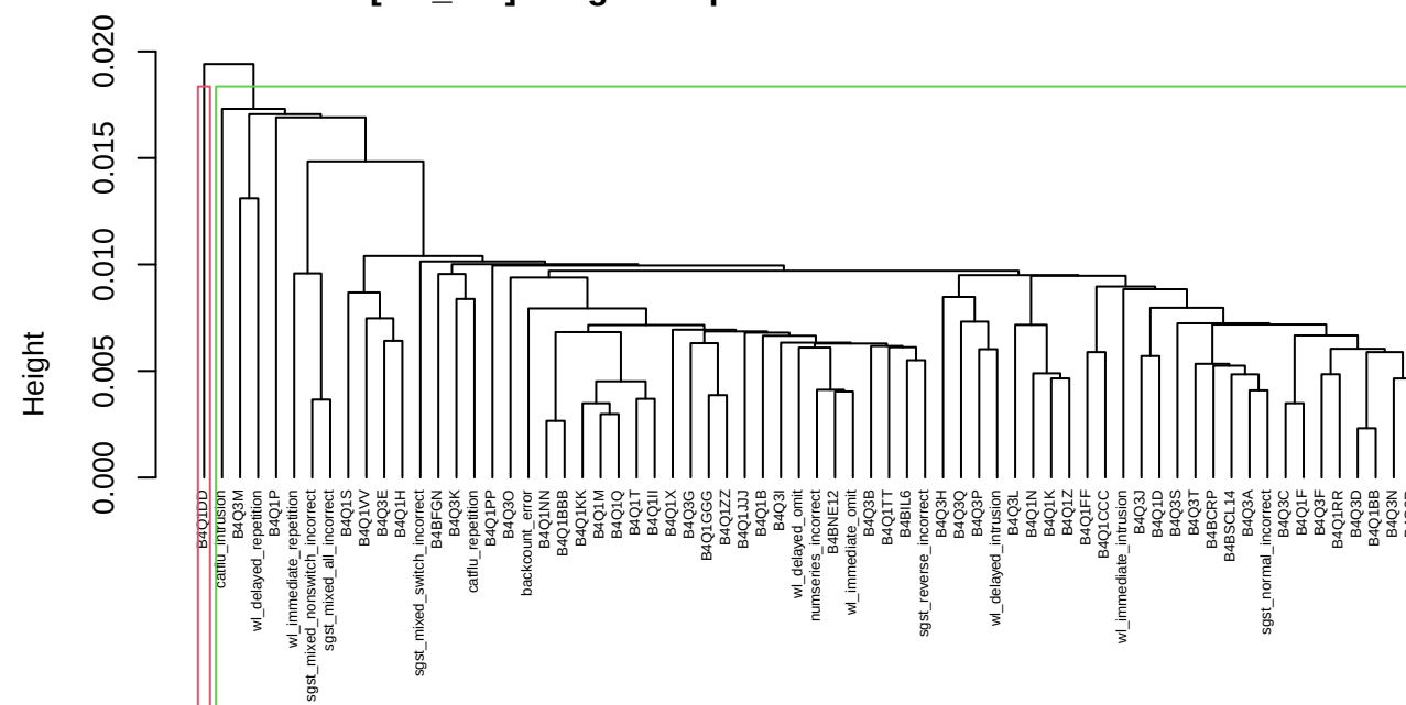
[eta PM] single coph=0.59 AC=0.67 K*=2 sil=0.26
