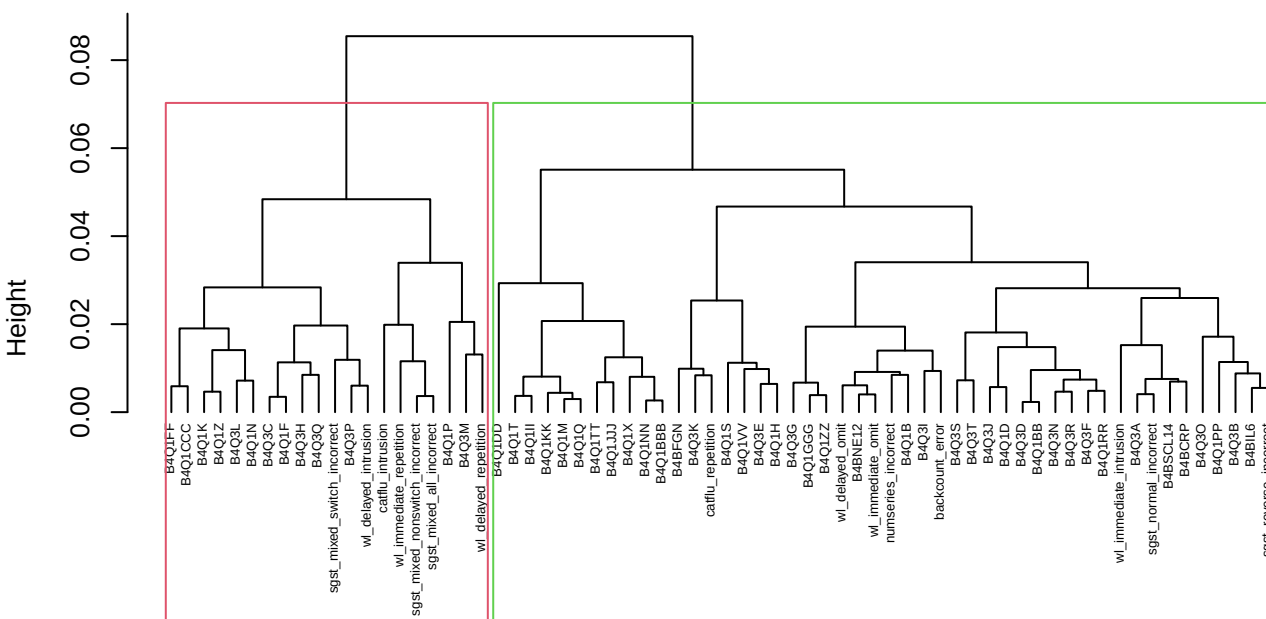
[eta PM] complete coph=0.69 AC=0.91 K*=2 sil=0.42
