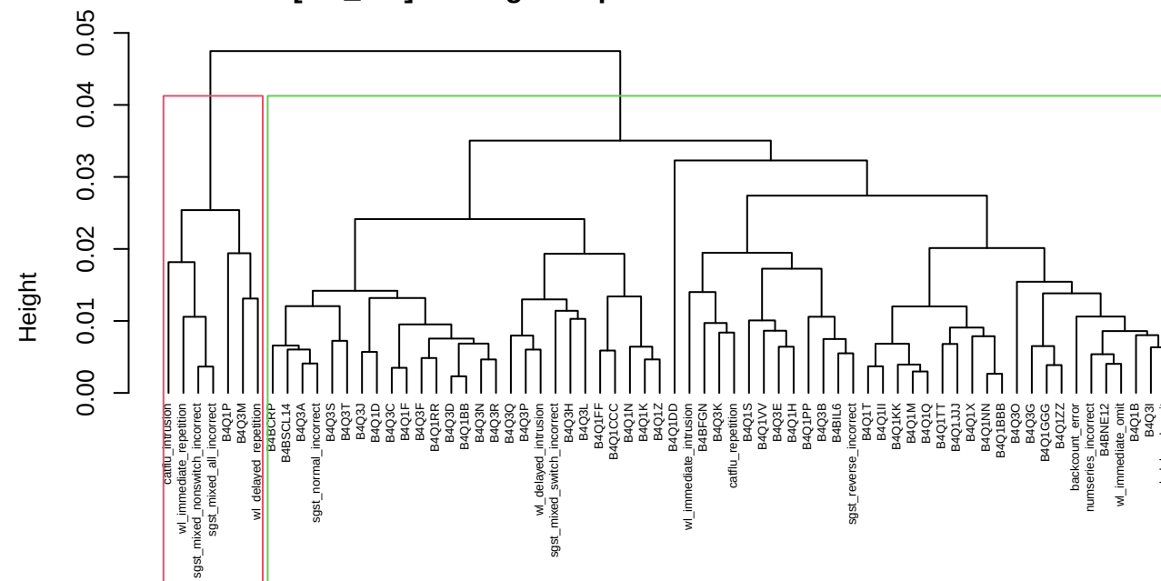
[eta_PM] average coph=0.69 AC=0.85 K*=2 sil=0.39
