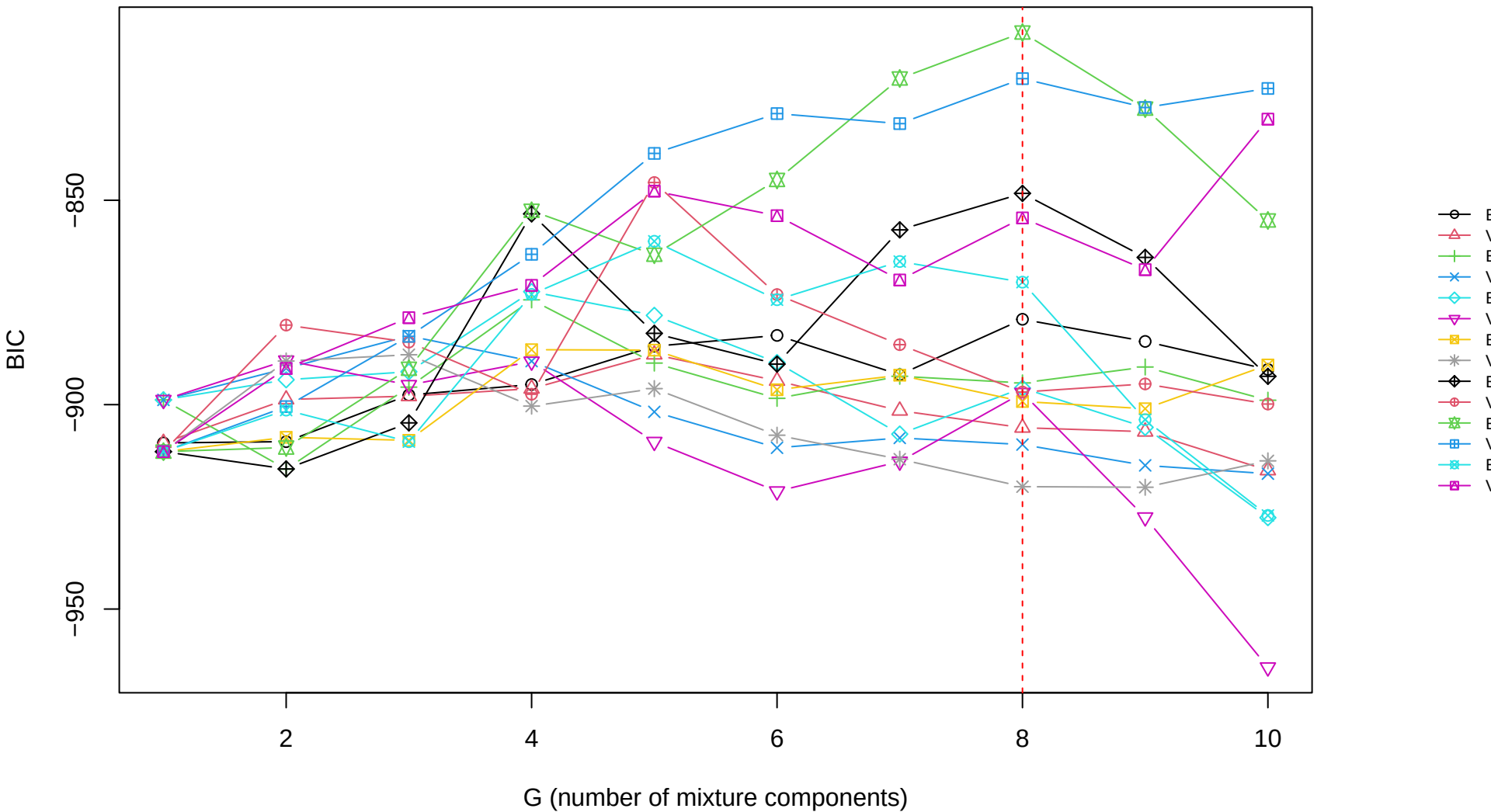
Mclust BIC sweep (best: G=8, EEV)
