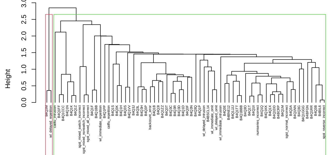
single (cophenetic = 0.65, AC = 0.78, K* = 2, sil = 0.23)
