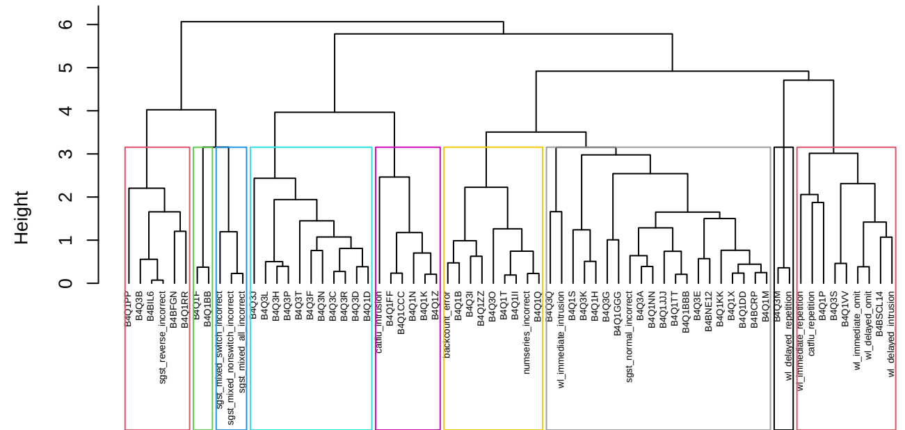
average (cophenetic = 0.70, AC = 0.88, K* = 9, sil = 0.40)
