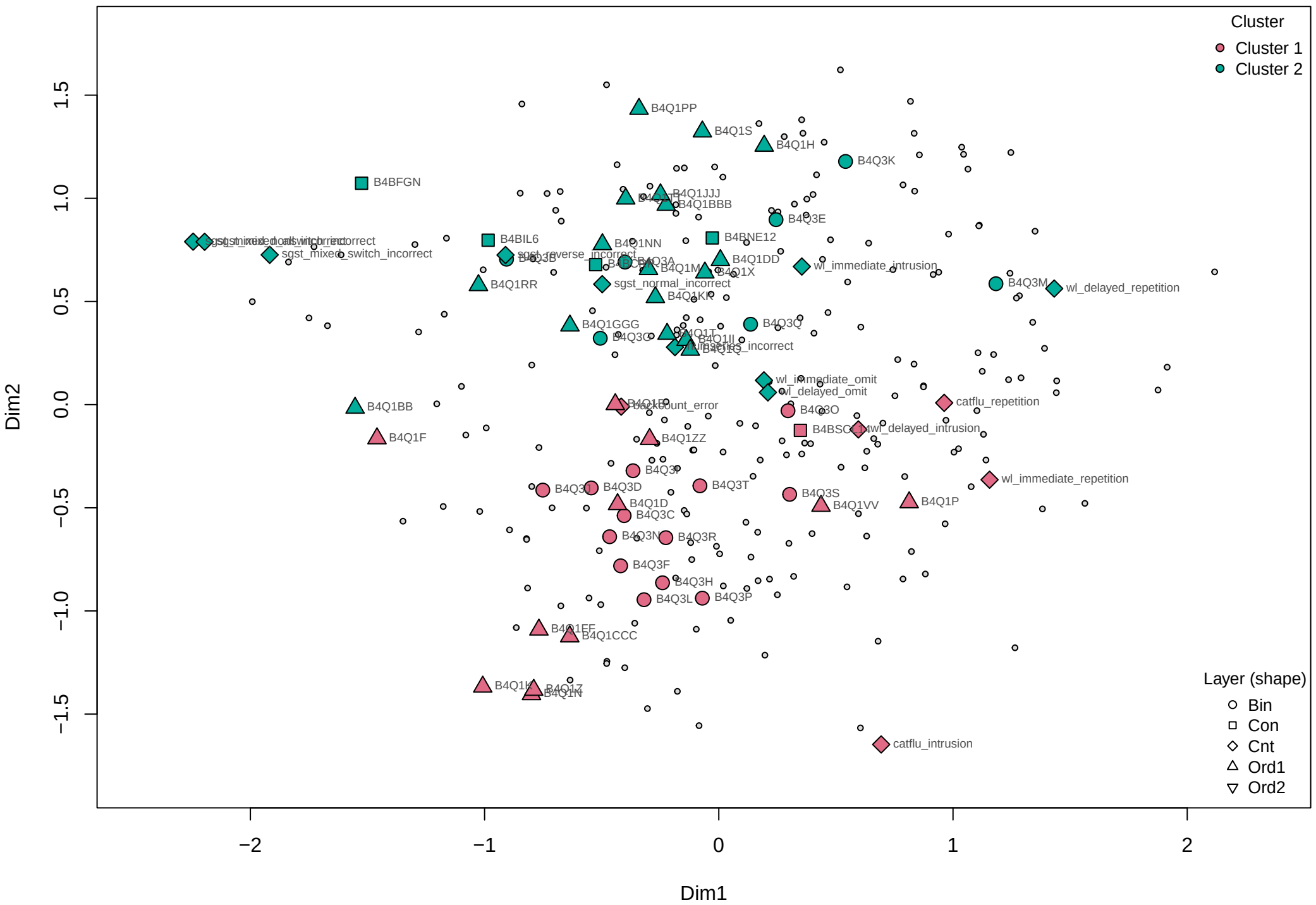
[K2] Item cluster membership (K=2, avg sil=0.360)
