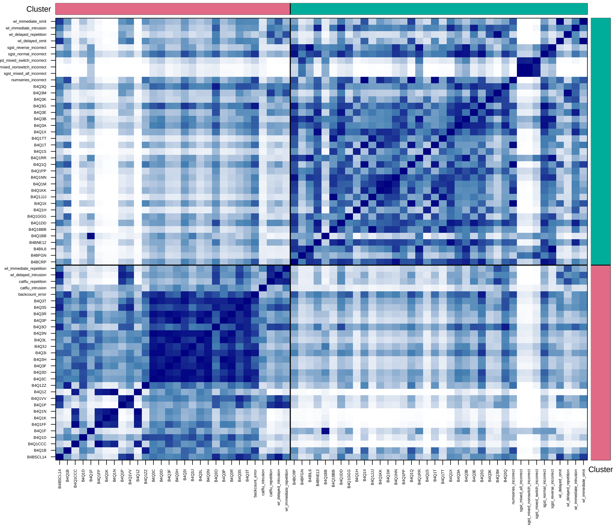
[K2] BC heatmap (M=68, K=2, avg sil=0.360)
