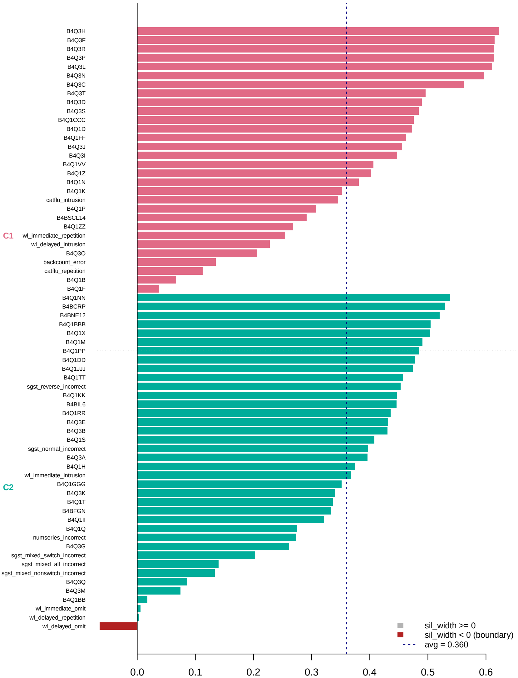
[K2] Per-item silhouette (K = 2, avg = 0.360)
