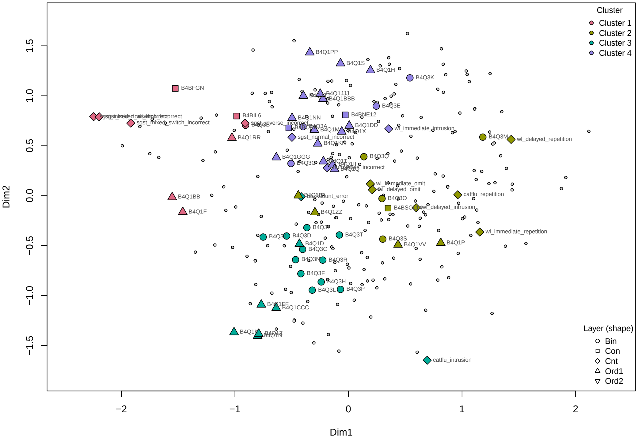
[K4] Item cluster membership (K=4, avg sil=0.404)
