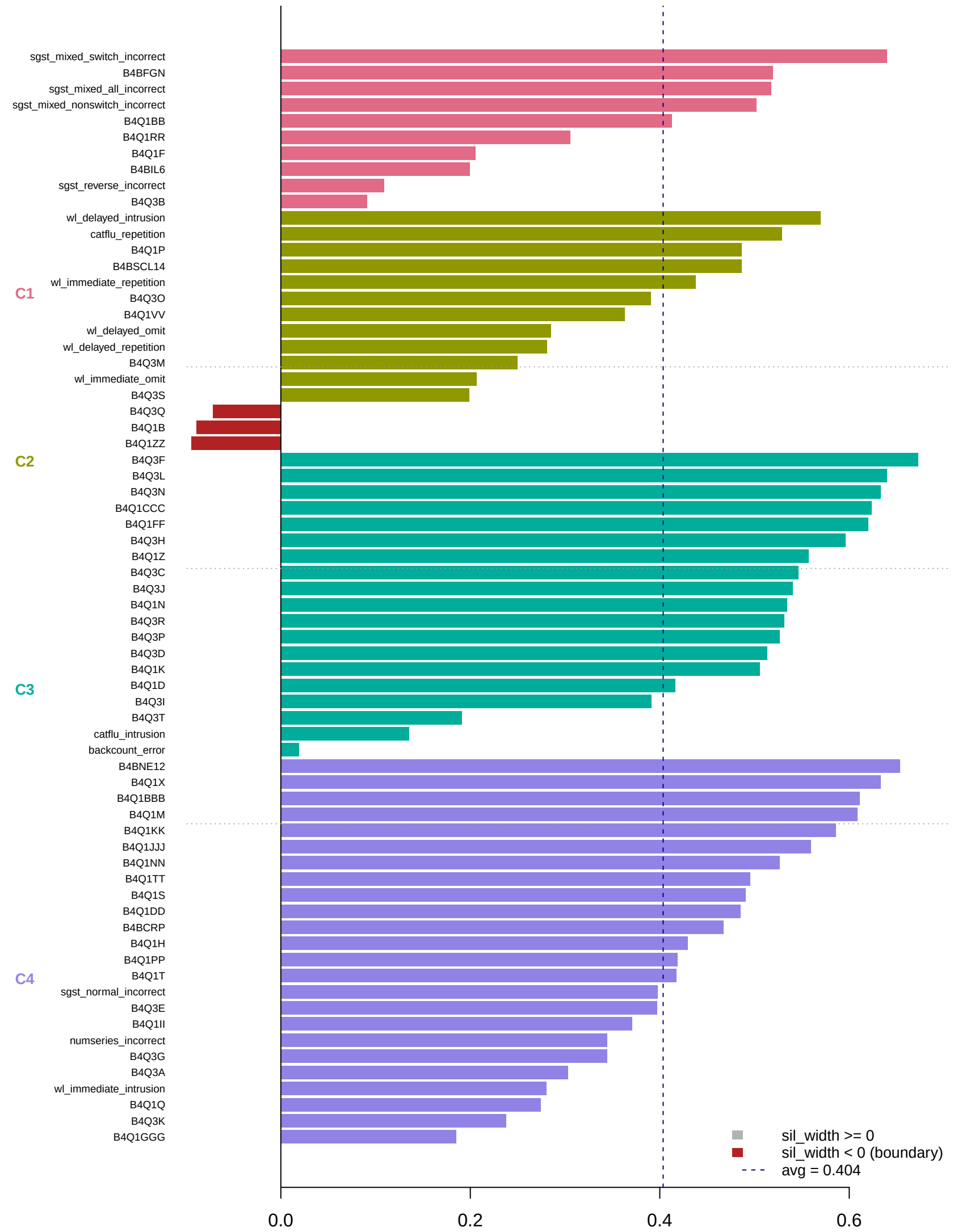
[K4] Per-item silhouette (K = 4, avg = 0.404)
