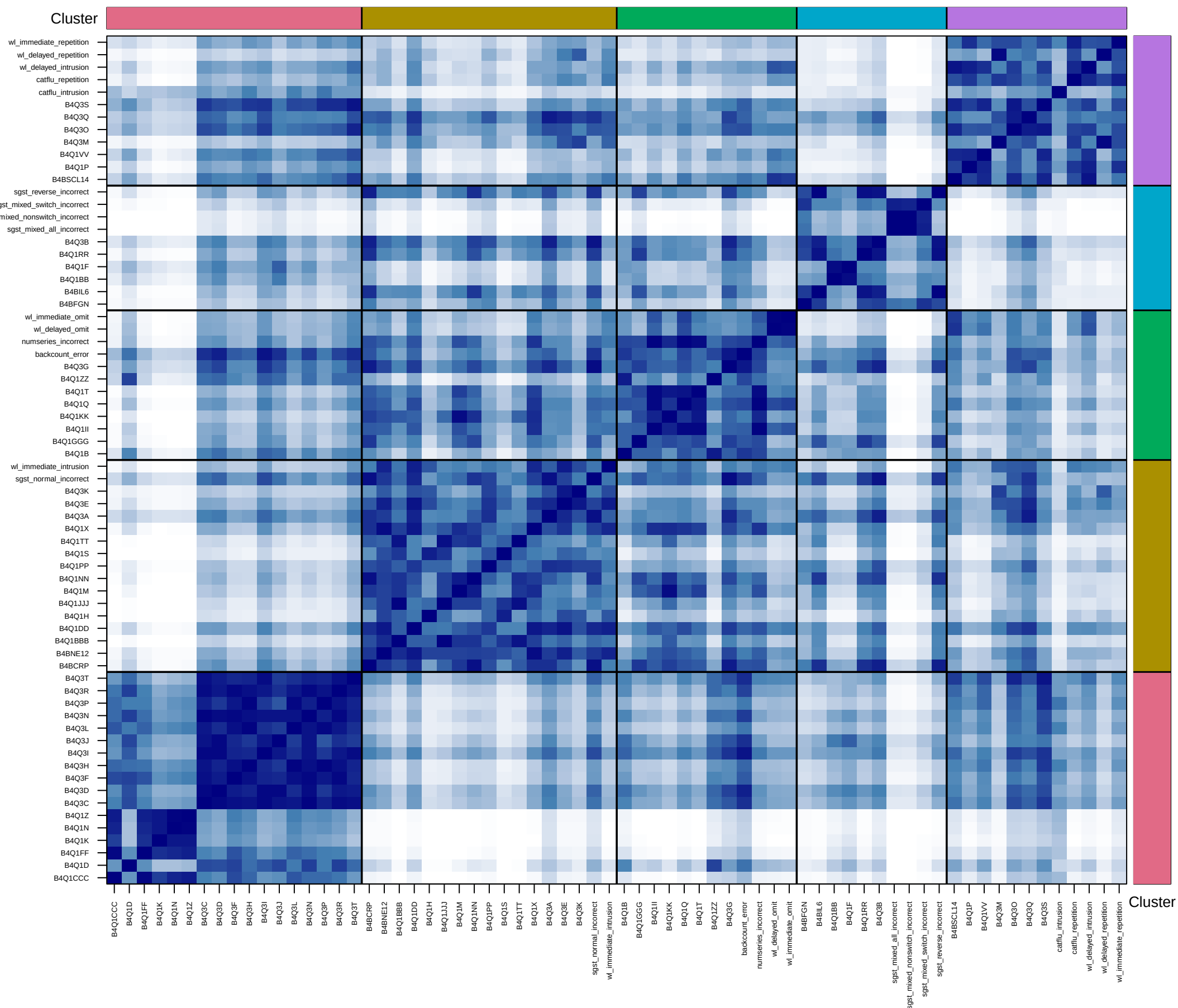
[K5] BC heatmap (M=68, K=5, avg sil=0.423)
