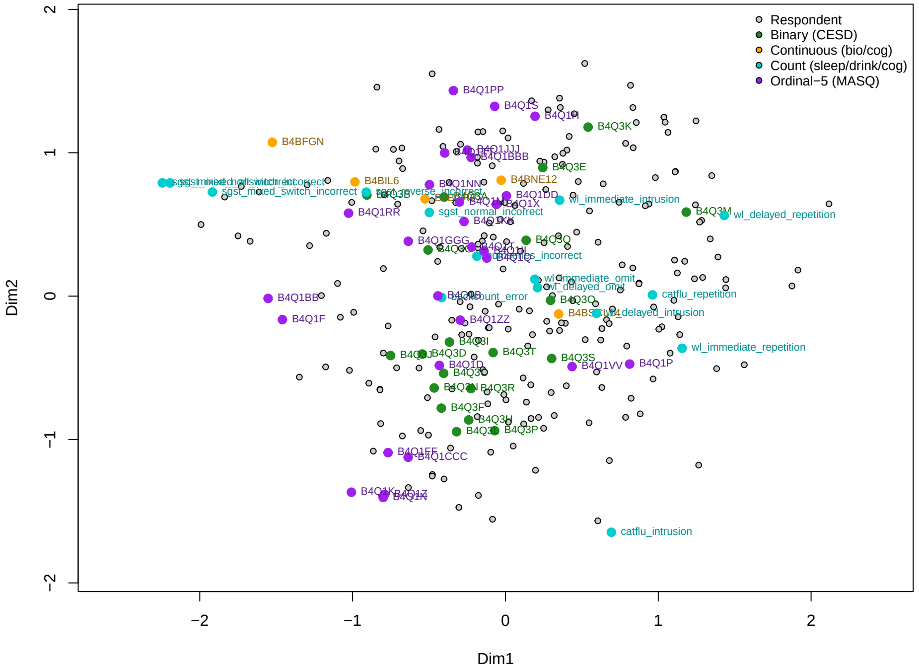
MIDUS W2+R1: Case 1: All (bin+con+cnt+ord) [con_inflammation_cnt_cognition_ord_all] (GRM v5)
