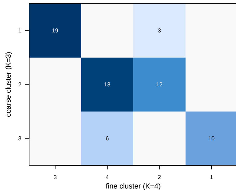
coarse K=3 x fine K=4 (ref = 0.87)
