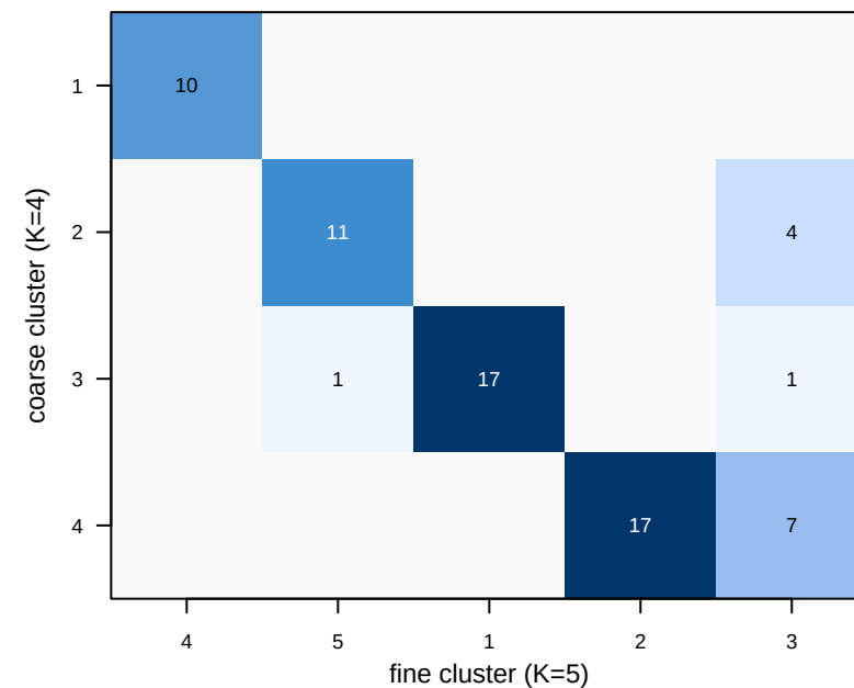
coarse K=4 x fine K=5 (ref = 0.91)
