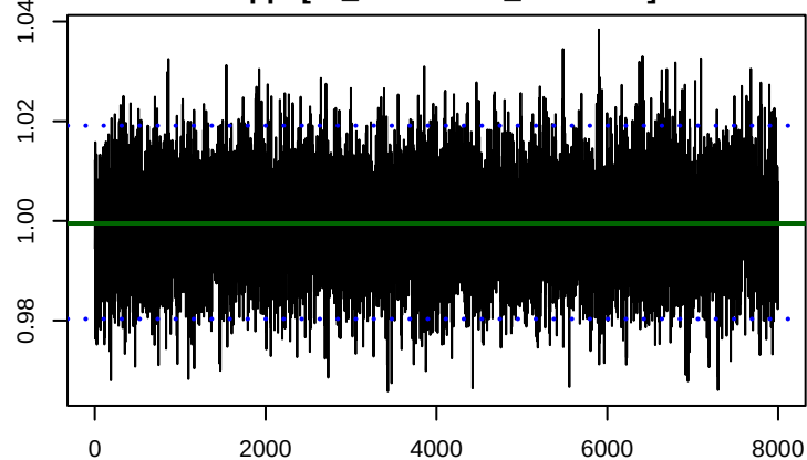
kappa[wl_immediate_intrusion]
