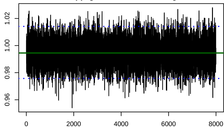
kappa[numseries_incorrect]
