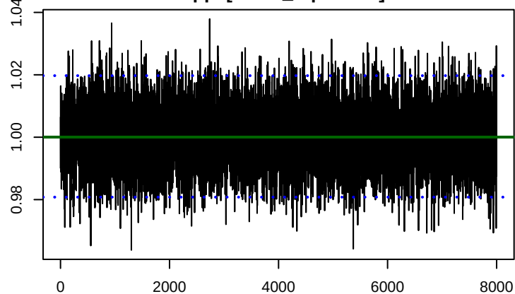
kappa[catflu_repetition]
