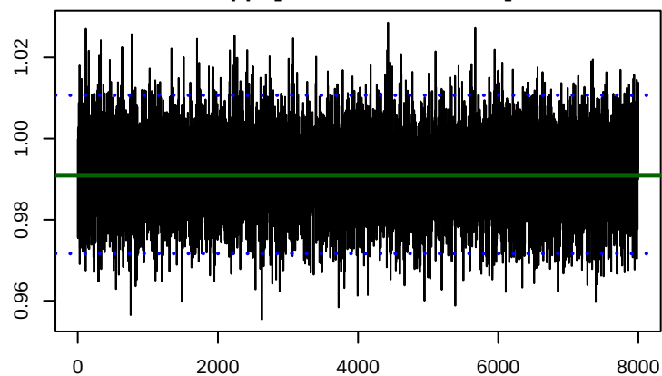
kappa[wl_immediate_omit]
