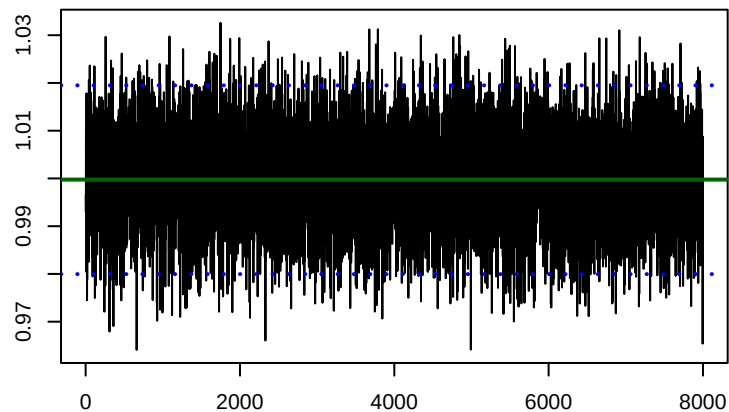
kappa[sgst_mixed_switch_incorrect]
