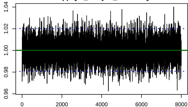
kappa[wl_delayed_intrusion]
