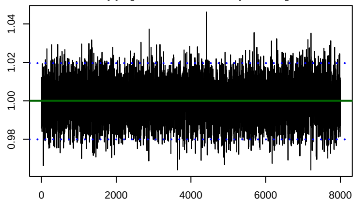
kappa[wl_immediate_repetition]
