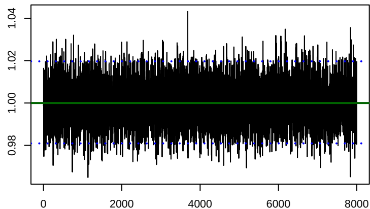
kappa[sgst_normal_incorrect]
