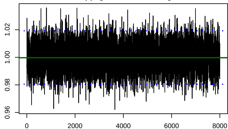
kappa[backcount_error]
