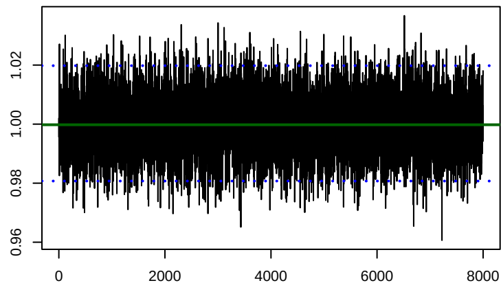
kappa[sgst_reverse_incorrect]
