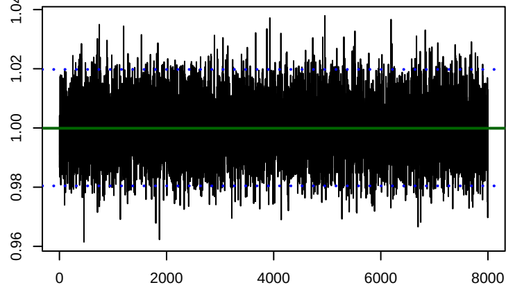
kappa[sgst_mixed_all_incorrect]
