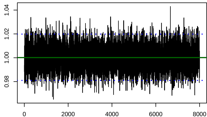
kappa[sgst_mixed_nonswitch_incorrect]
