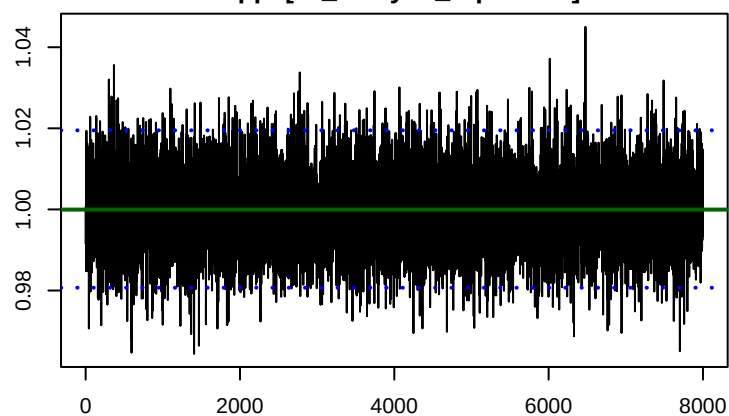
kappa[wl_delayed_repetition]
