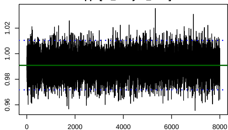
kappa[wl_delayed_omit]
