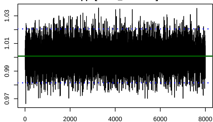
kappa[catflu_intrusion]
