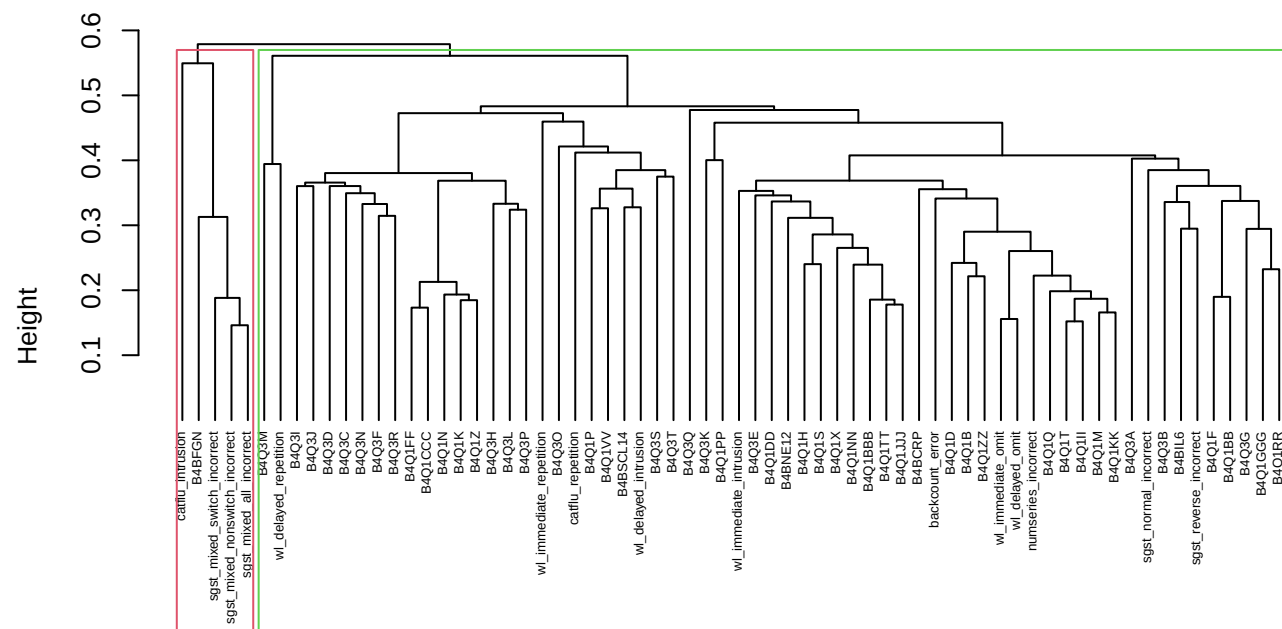
[D_bar] average coph=0.77 AC=0.50 K*=2 sil=0.23
