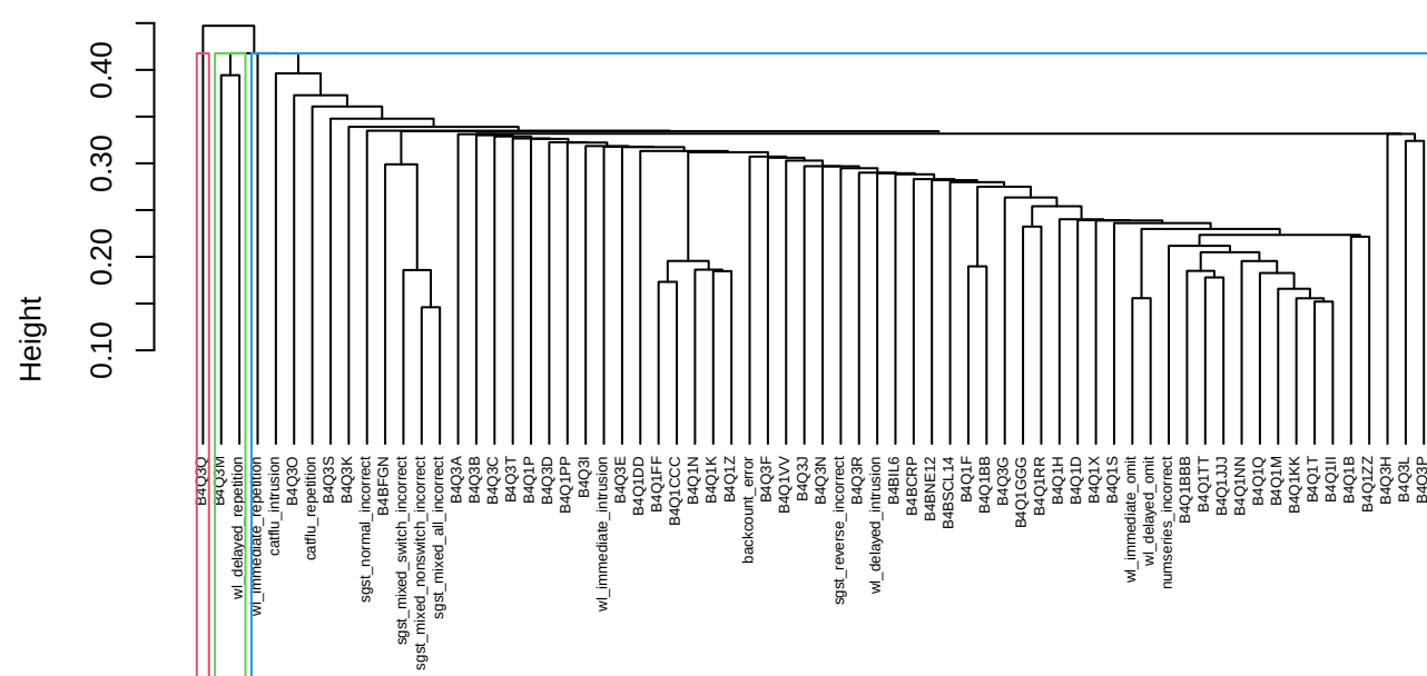
[D_bar] single coph=0.58 AC=0.40 K*=3 sil=0.08
