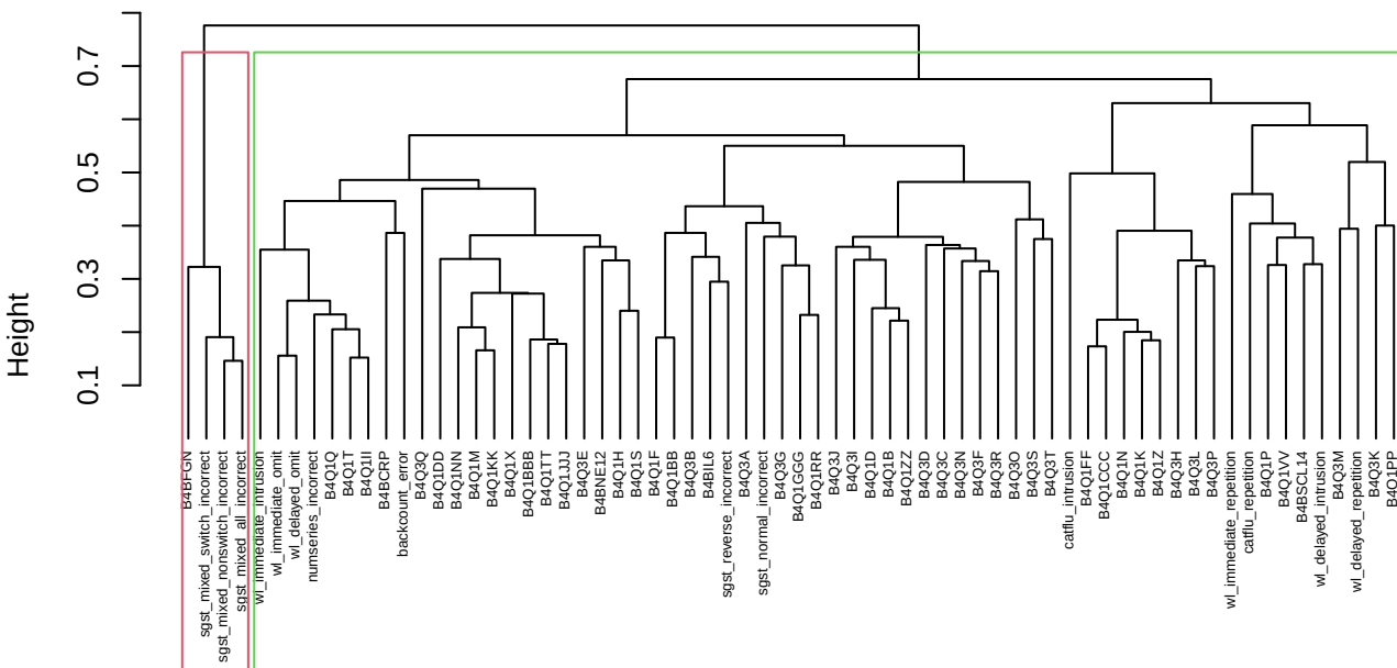
[D_bar] complete coph=0.70 AC=0.63 K*=2 sil=0.23
