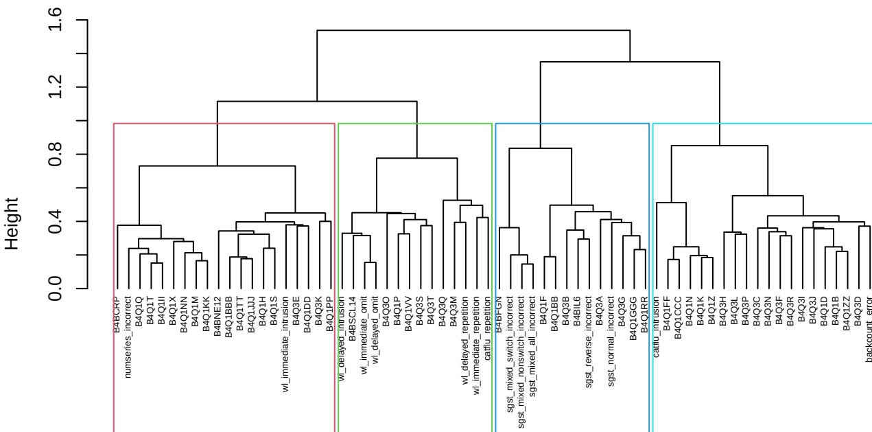
[D_bar] ward.D2 coph=0.54 AC=0.81 K*=4 sil=0.15
