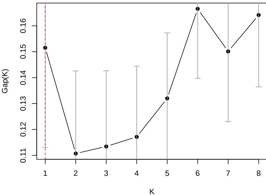
Gap (Tibs2001SEmax): K=1
