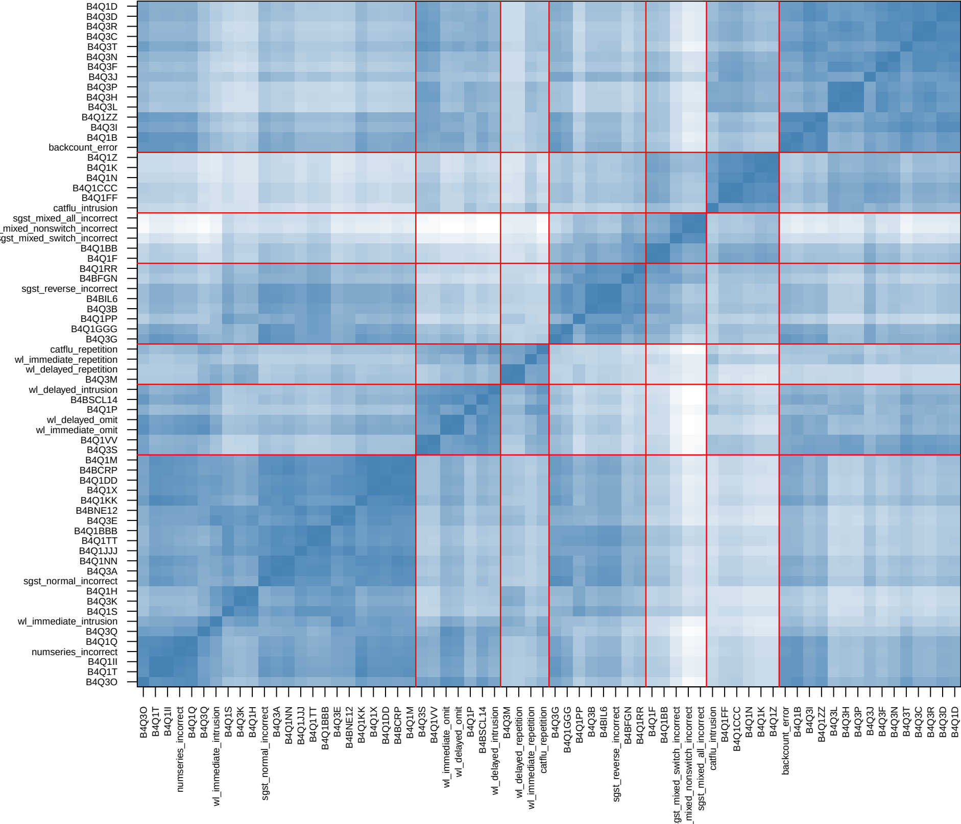
Pairwise distance heatmap reordered by ward.D2 (K* = 7)
