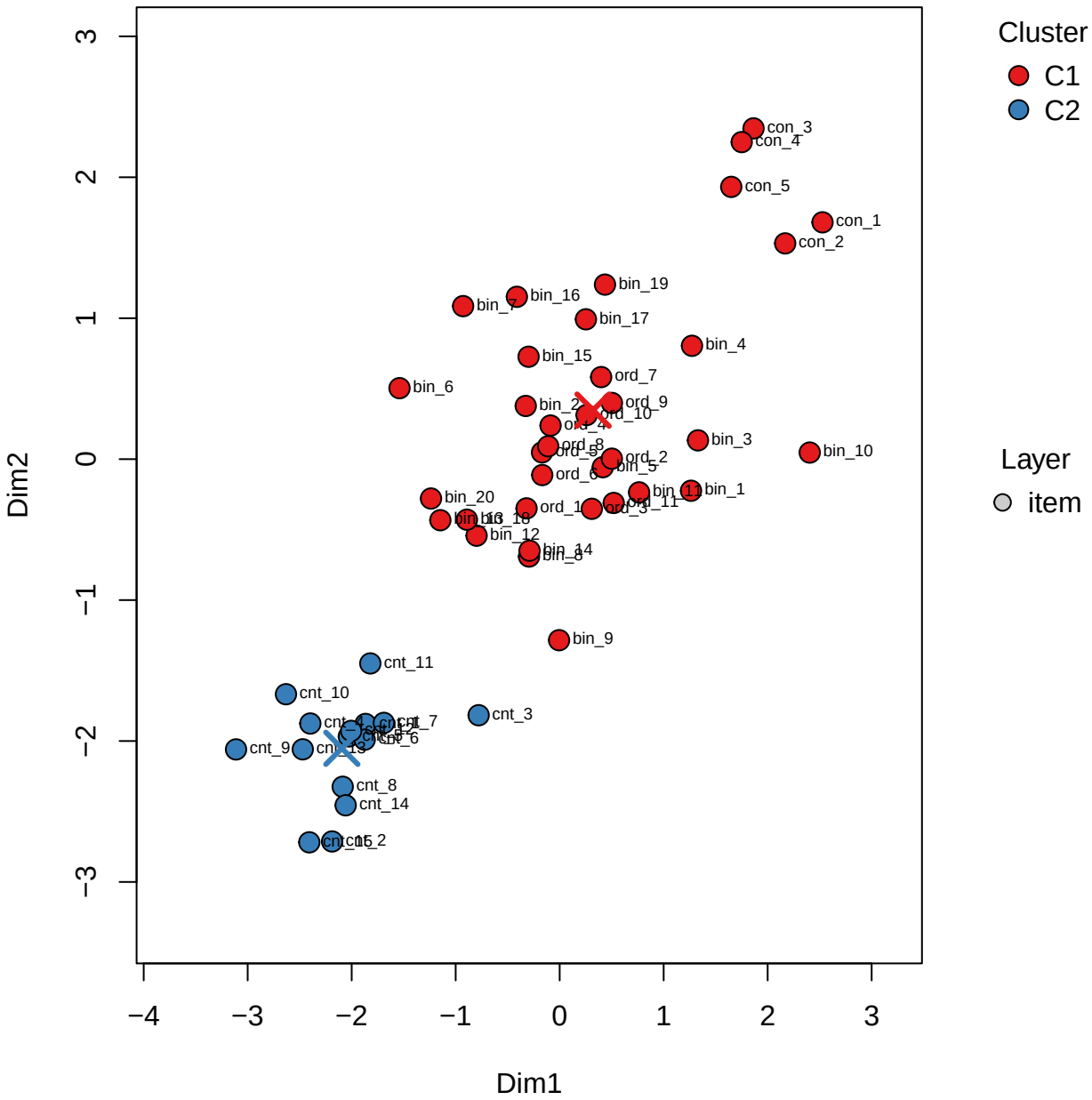
K-means on b (K=2, avg silhouette=0.576)
