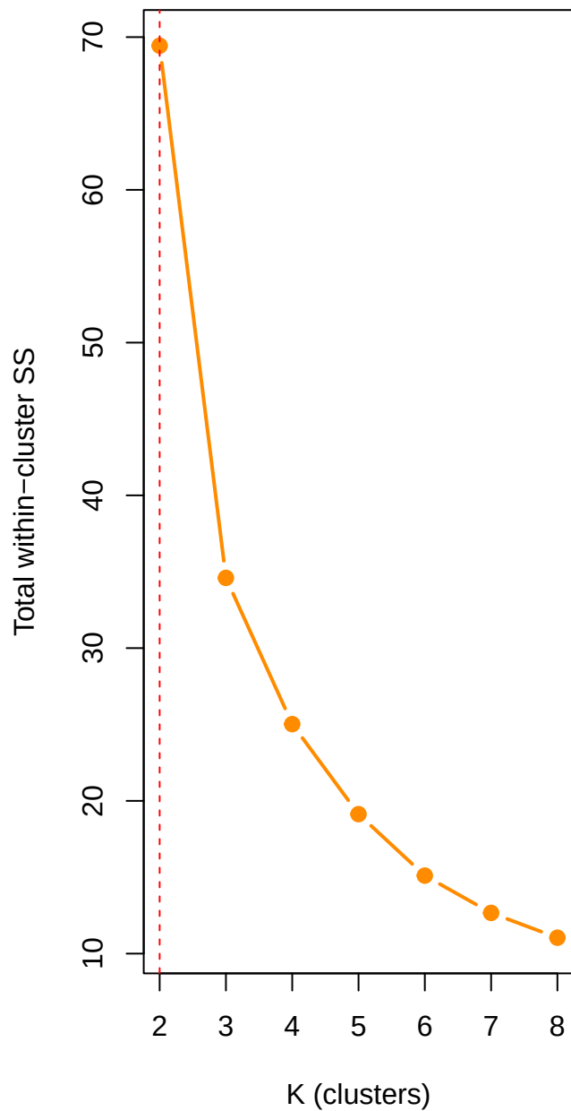
Elbow: within-SS vs K
