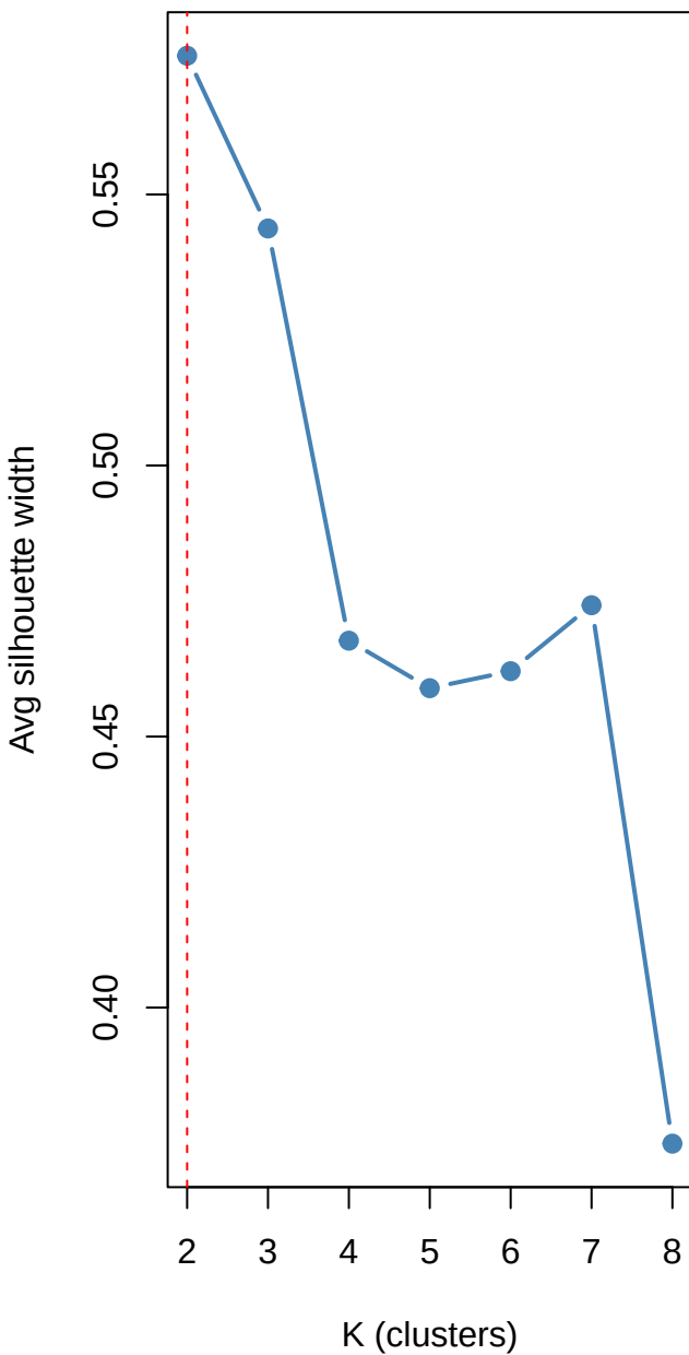
Silhouette vs K
