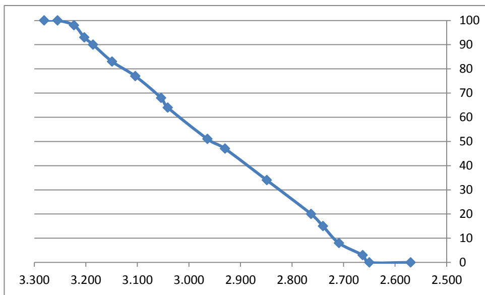
Battery voltage – Battery Percent (MCU reported)
