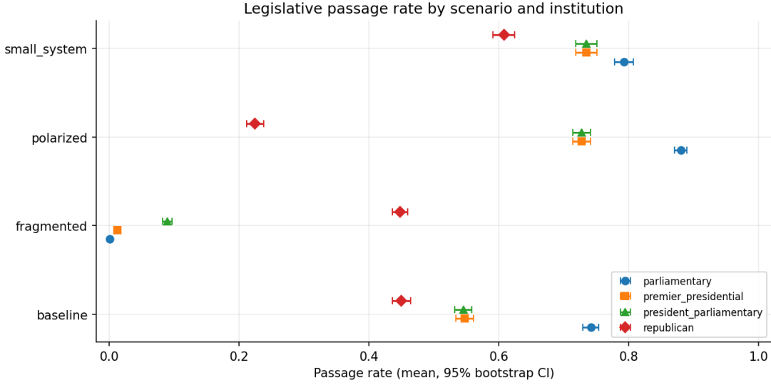
Figure 1: Mean passage rate with 95% bootstrap confidence intervals across four institutions and four scenarios ( N = 200 seeds per cell). The baseline parliamentary advantage reverses under fragmentation: pure parliamentary and premier-presidential collapse to near-zero passage, while president-parliamentary partially rescues and republican is unaffected. Section 4.1 reports the full passage-rate table; Section 4.4 attributes the collapse to party discipline.
