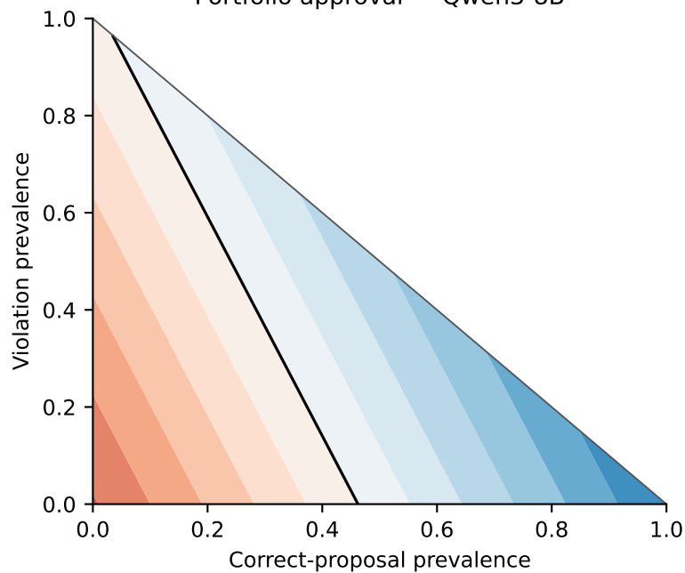
Portfolio approval — Qwen3-8B
