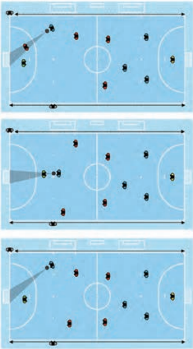
Goal unguarded
