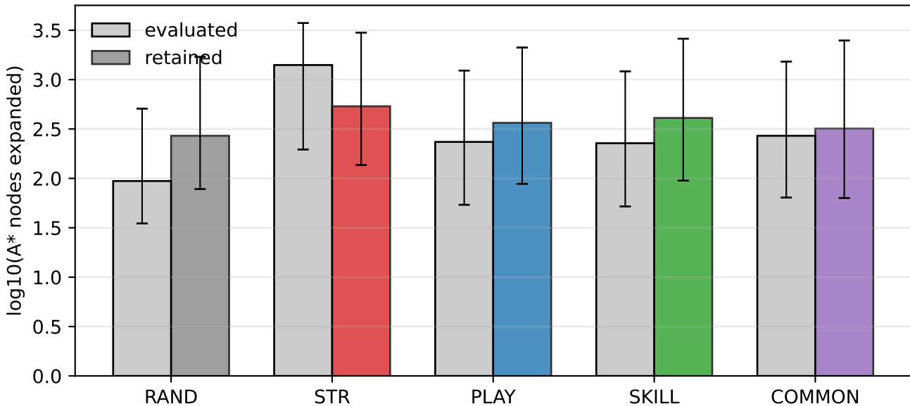
Implicit hardness selection: evaluated vs retained elites — Sokoban
