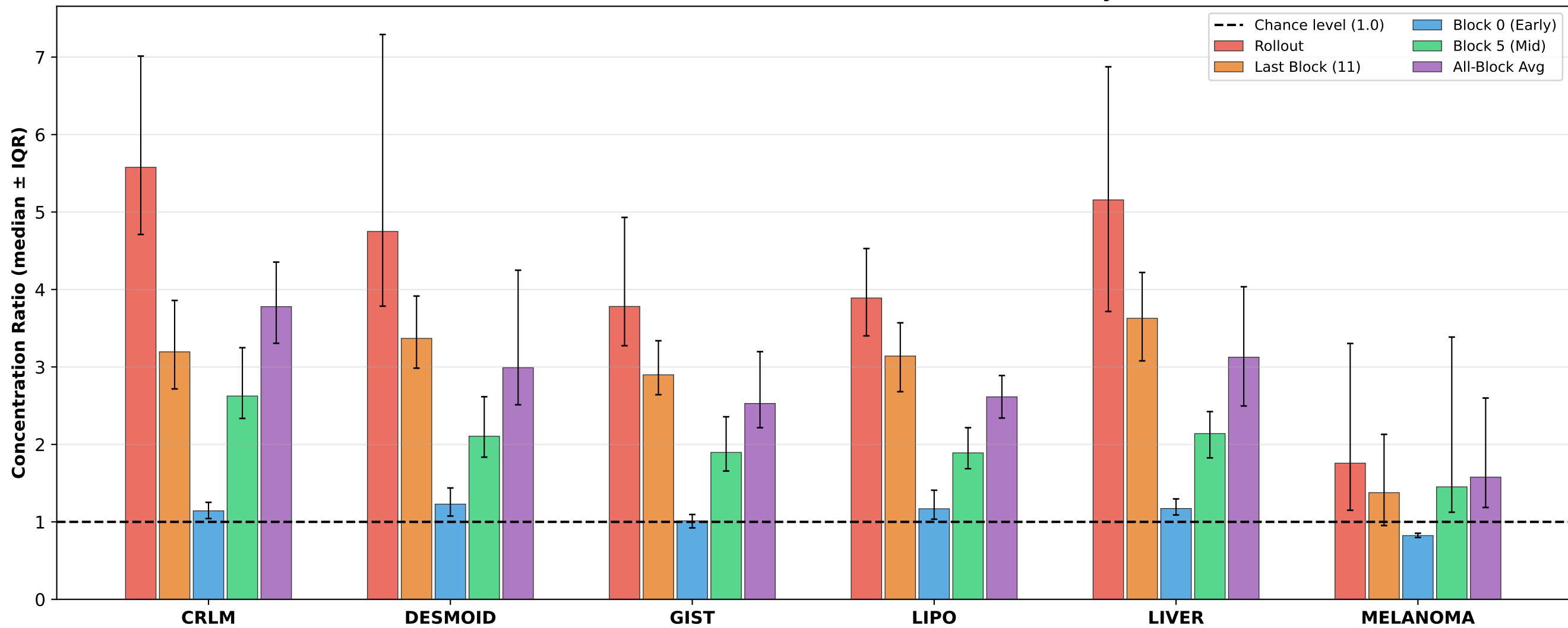
SAM-Med3D — Attention Concentration in Lesion (Normalized by Lesion Size)
