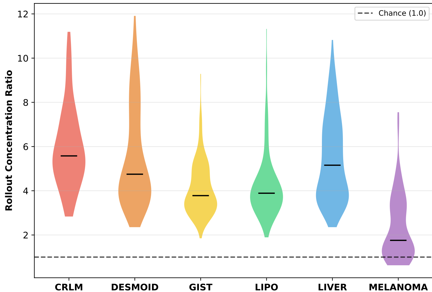
Attention Concentration (>1 = lesion-focused)
