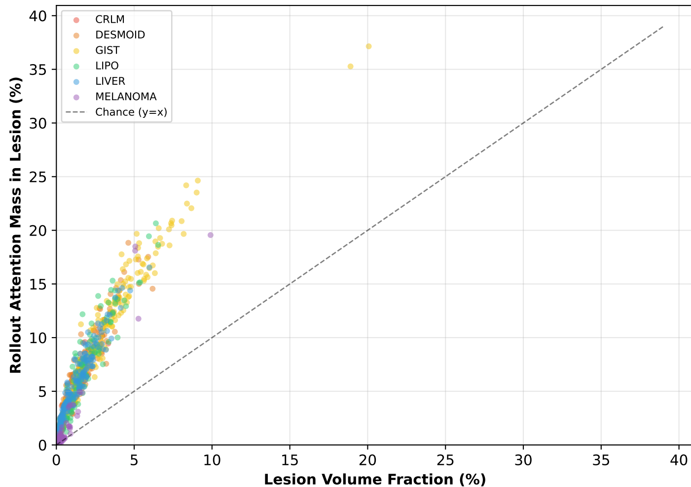
Lesion Volume vs. Attention Mass (Rollout)
