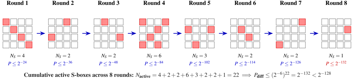
Figure 2: Visualization of the optimal 8-round differential characteristic trail for Rubik-4D obtained by MILP solver. Each 4 \times 4 grid represents the 16-byte state, where shaded red squares designate active S-boxes. The cascade demonstrates that the cumulative active S-box lower bound reaches N_{\text{active}} = 22 , bounding the maximum differential probability to P_{\text{diff}} \leq 2^{-132} .
