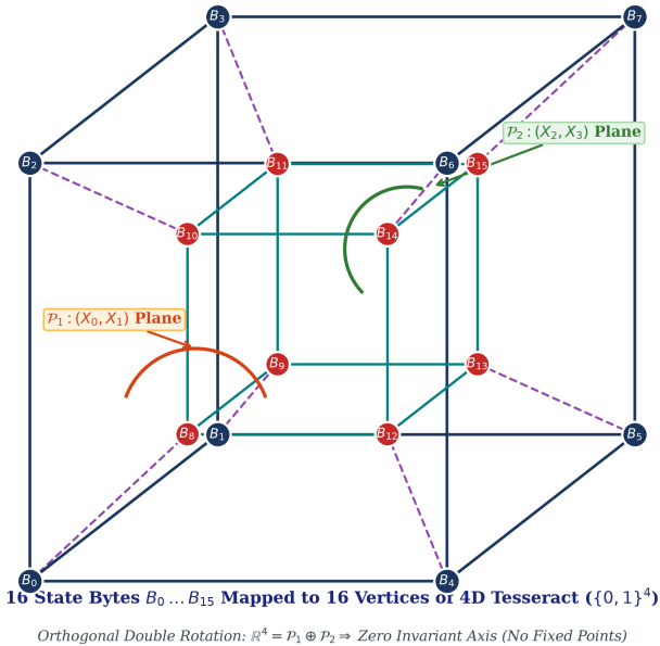
Figure 1: Geometric representation of the Rubik-4D 128-bit internal state over a four-dimensional hypercube (tesseract, \{0,1\}^4 ). State bytes B_0 \dots B_{15} are mapped to 16 distinct vertices. Discrete double orthogonal rotations from Lie group SO(4) act simultaneously across pairs of orthogonal 2D planes (e.g., \mathcal{P}_1 and \mathcal{P}_2 ), avoiding invariant axes and ensuring full coordinate mixing.
