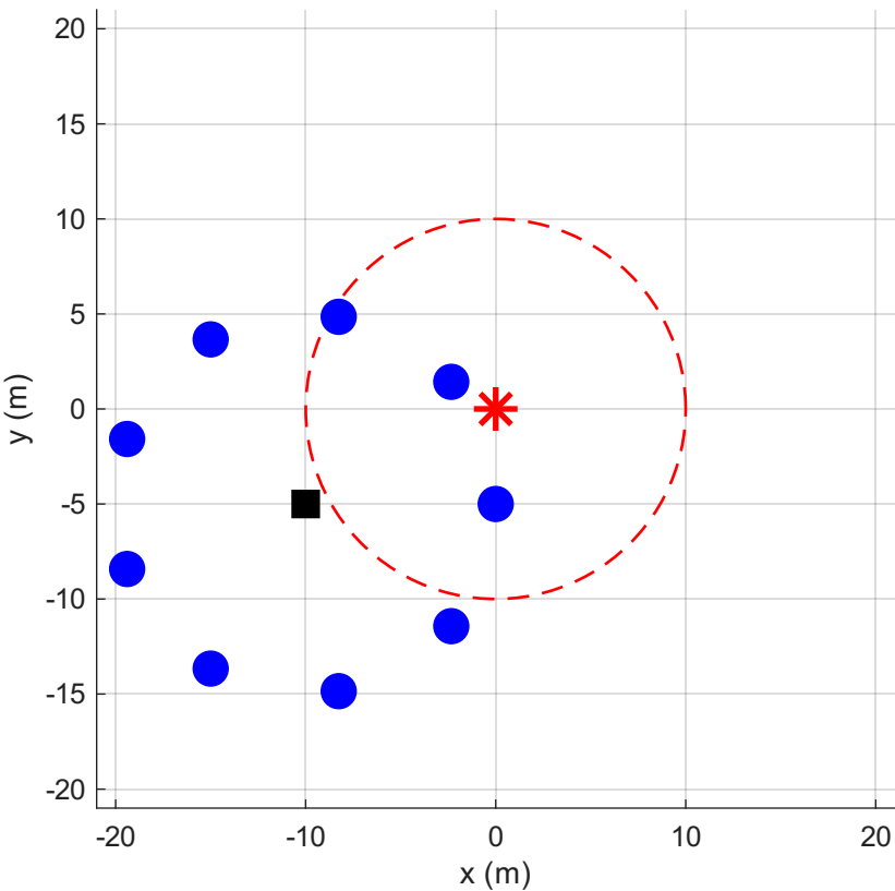
Initial: N_{\text{obs}} = 3
